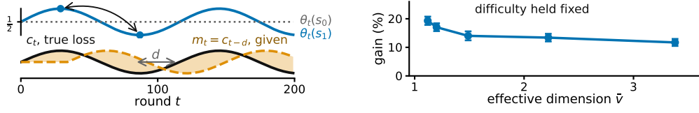
Figure 1: An illustration of the two things that limit intermediate feedback, on generated data. Left , what each state predicts about the outcome changes while the map from choices to states stays fixed, so the losses from d rounds earlier grow increasingly inaccurate; E_2 of Section 3 tracks that. Right , more overlap between choices allows more sharing, at matched difficulty, K = 40 , |\mathcal{S}| = 8 , T = 10000 , d = 50 , 20 paired seeds, bars one standard error of the paired difference (Appendix I, study 10).
