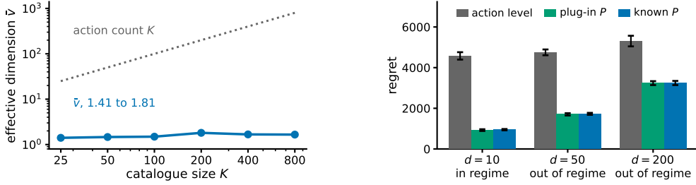
Figure 4: Experiment 3, a recommendation funnel. Left , the effective dimension stays near two while the catalogue grows thirty-two-fold, so the gap between K and \bar{v} comes from the catalogue having categories, not from a chosen K . Right , the three arms at T = 20000 and 8 paired seeds, labelled by whether \bar{v}(d+1) \log K \leq K + d holds. Bars are one standard error. No real data is used anywhere in this experiment.
