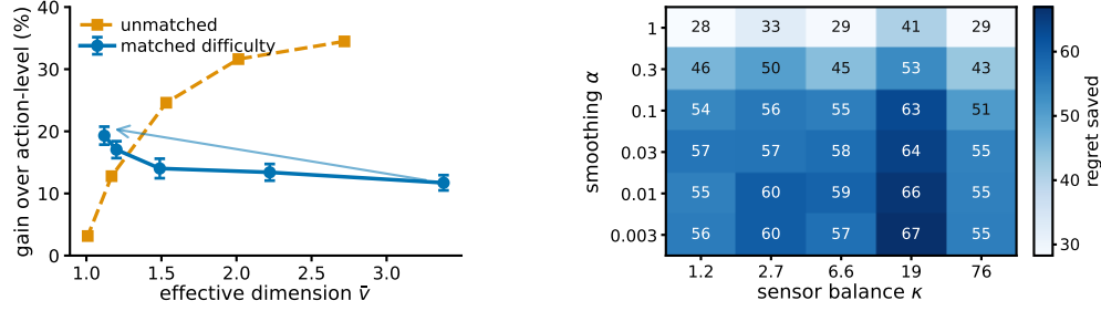
Figure 3: Left , Experiment 2. The same overlap sweep with and without holding the task difficulty fixed. Matching the uniform-play regret reverses the trend, supporting the interpretation that the decline in the unmatched sweep is driven by task-difficulty confounding rather than by the pooling mechanism itself. Bars are one standard error of the paired difference. Right , regret saved against action-level weighting as the smoothing pseudocount used to estimate P and the sensor balance vary, with 10 paired seeds per cell; this is the sensitivity study using an estimated (plug-in) P , whose script is released with the rest.
