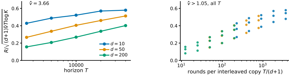
Figure 4: Study 9, the state channel. The plotted ratio would be flat if Theorem 1 captured the dependence on all three of T , d and \hat{v} . Left , horizon sweep at the largest effective dimension, one line per delay. Right , every cell with \hat{v} > 1.05 against rounds per interleaved copy, where the three delays fall on one curve.
