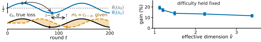
Figure 1: The claim and its boundary, on generated data. Left , what each state predicts changes while the action-to-state map stays fixed, so losses from d rounds earlier grow inaccurate; E_2 of Section 2 tracks it. Right , more overlap allows more sharing, at matched difficulty, K = 40 , |\mathcal{S}| = 8 , T = 10000 , d = 50 , 20 paired seeds, bars one standard error of the paired difference (Appendix E, study 10).
