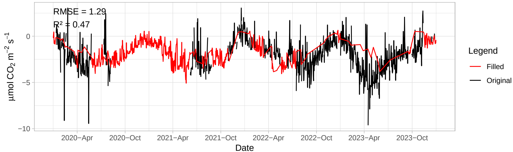
Actual vs Filled Carbon Dioxide Over Time
