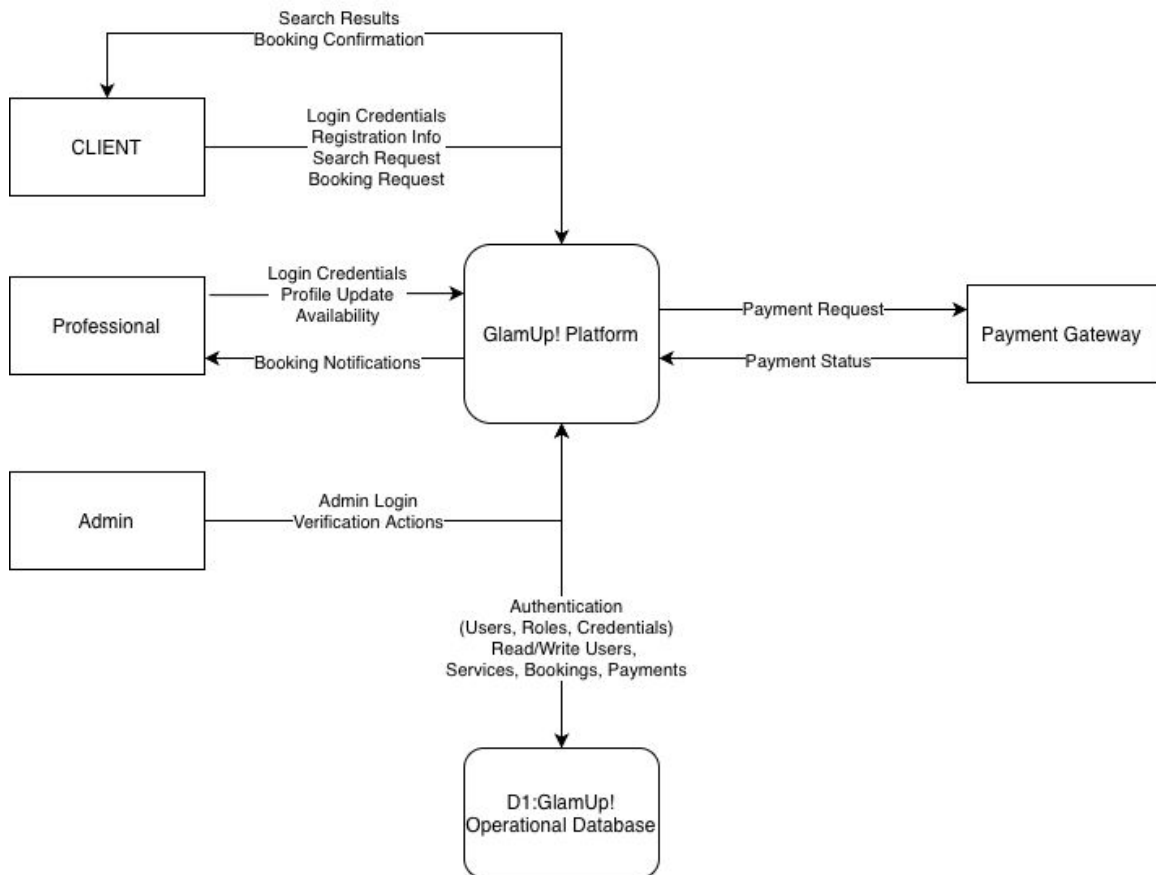
Level 0 Data Flow Diagram – GlamUp Platform
