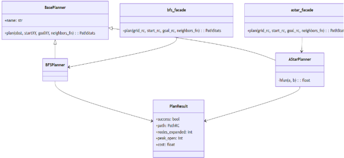
Figure III. Class diagram of algorithm modules, showing BFS and A* planners inheriting from a common base planner interface. *
