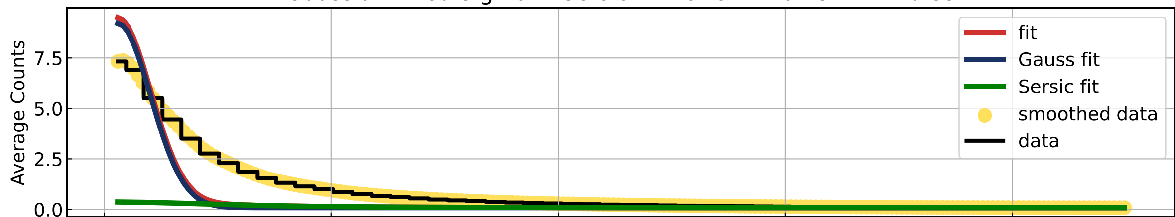
Guassian Fixed Sigma + Sersic Min One N -- 0.75 < z < 0.85
