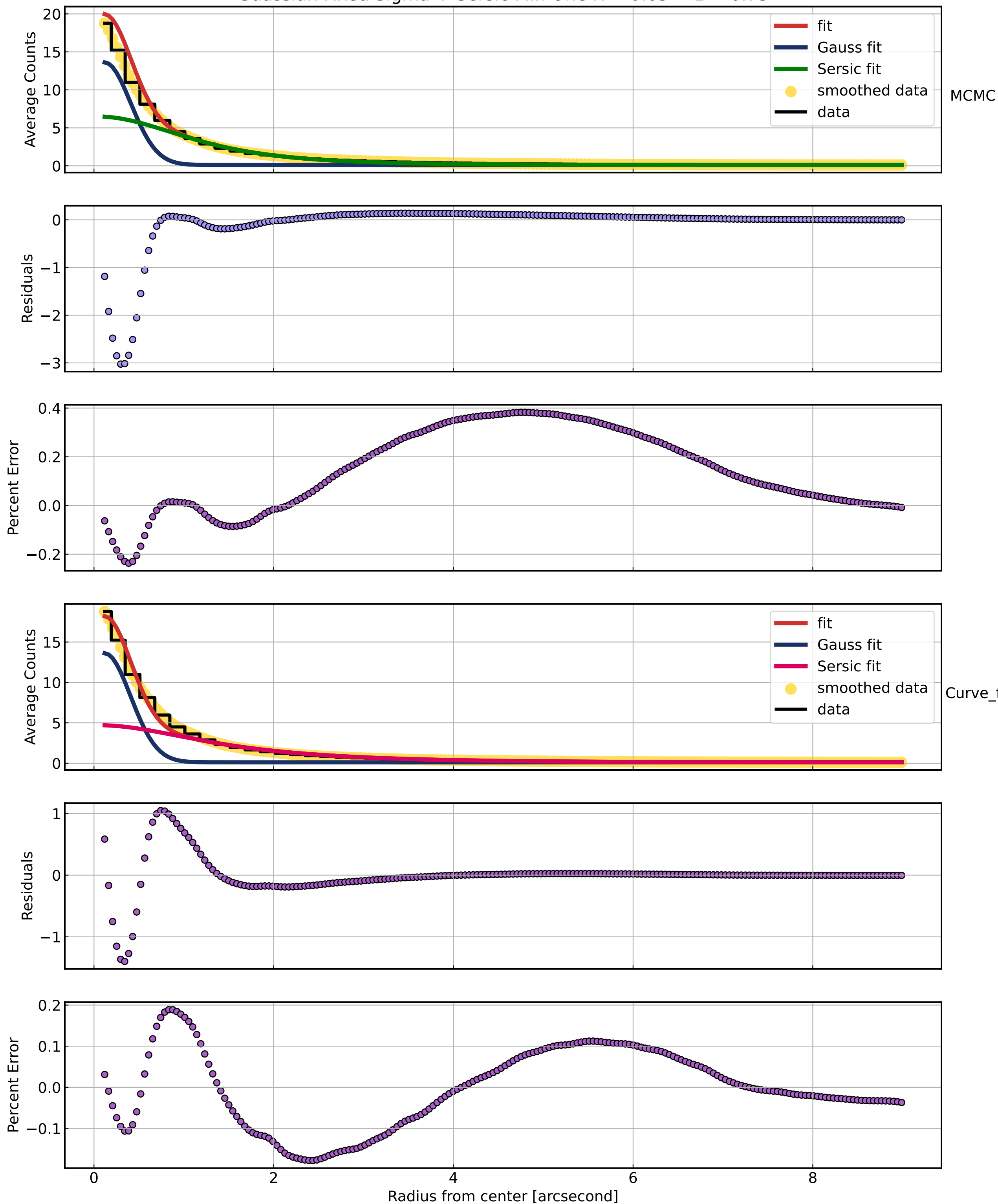
Guassian Fixed Sigma + Sersic Min One N -- 0.65 < z < 0.75
