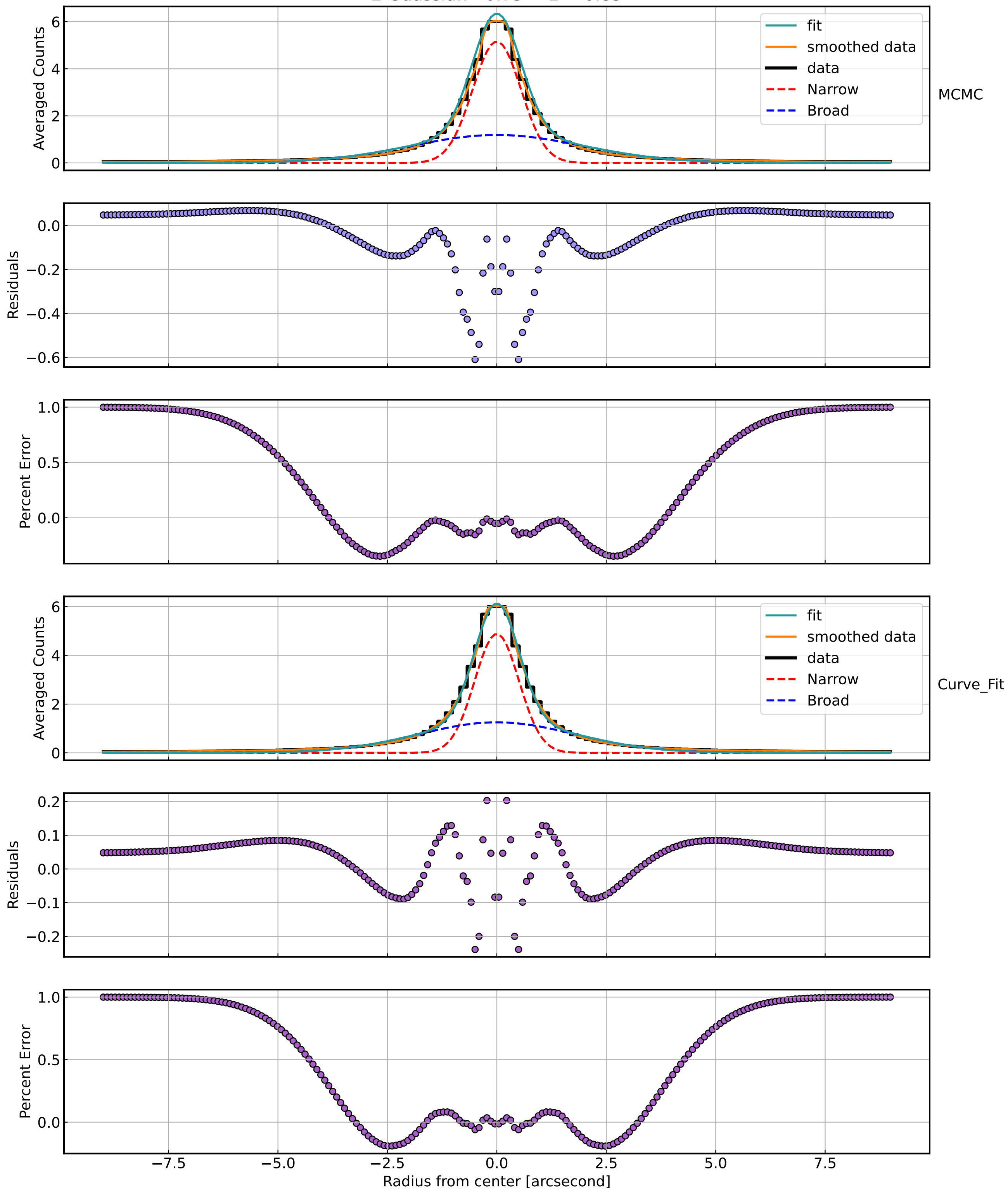
2 Guassian - 0.75 < z < 0.85
