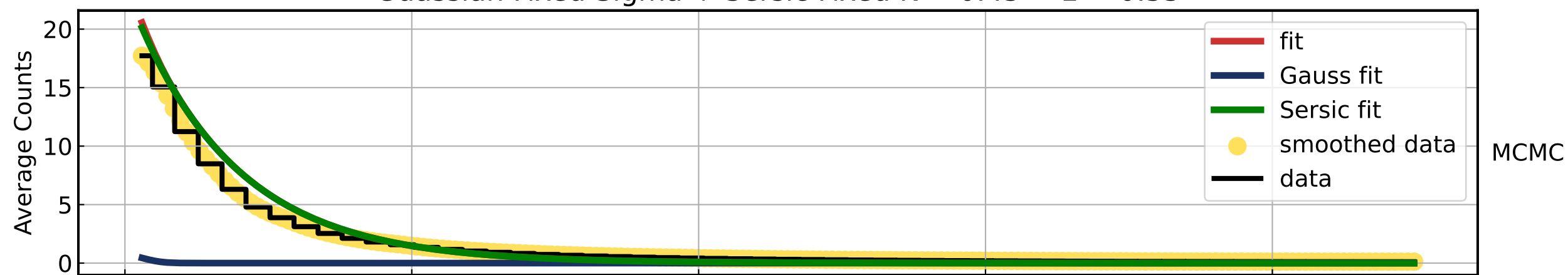
Guassian Fixed Sigma + Sersic Fixed N -- 0.45 < z < 0.55
