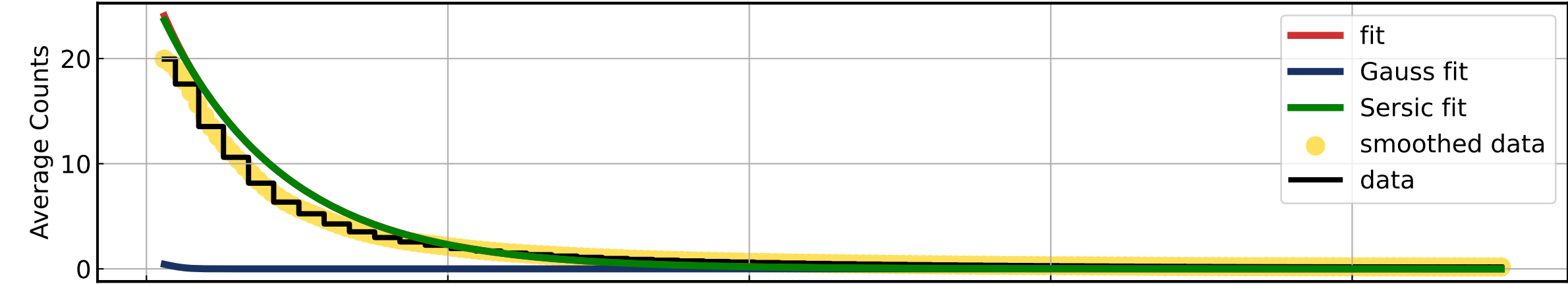
Guassian Fixed Sigma + Sersic Fixed N -- 0.35 < z < 0.45
