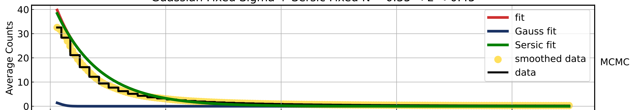
Guassian Fixed Sigma + Sersic Fixed N -- 0.35 < z < 0.45
