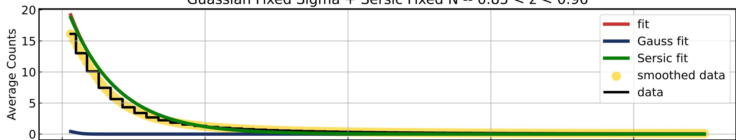
Guassian Fixed Sigma + Sersic Fixed N -- 0.85 < z < 0.96
