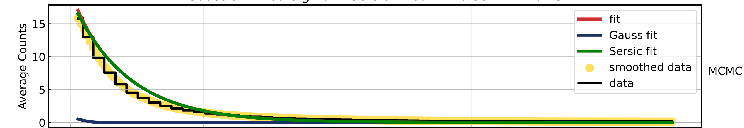
Guassian Fixed Sigma + Sersic Fixed N -- 0.35 < z < 0.45
