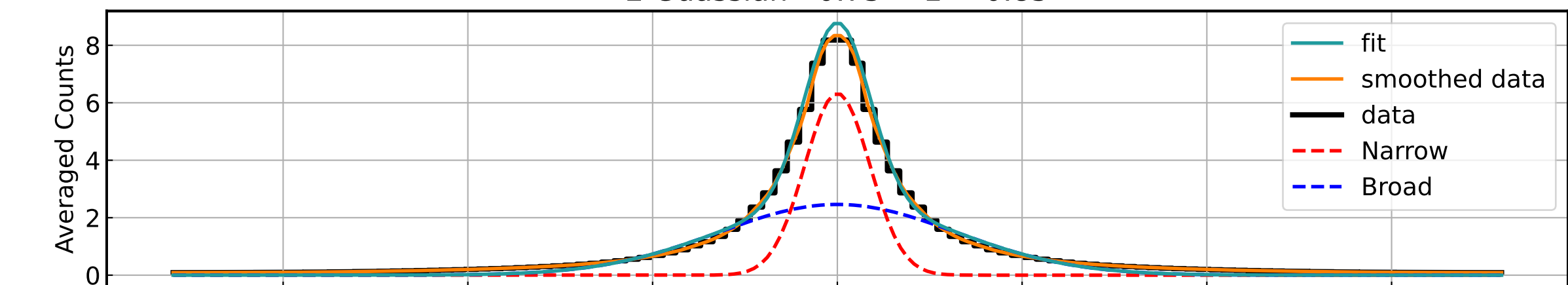
2 Guassian - 0.75 < z < 0.85
