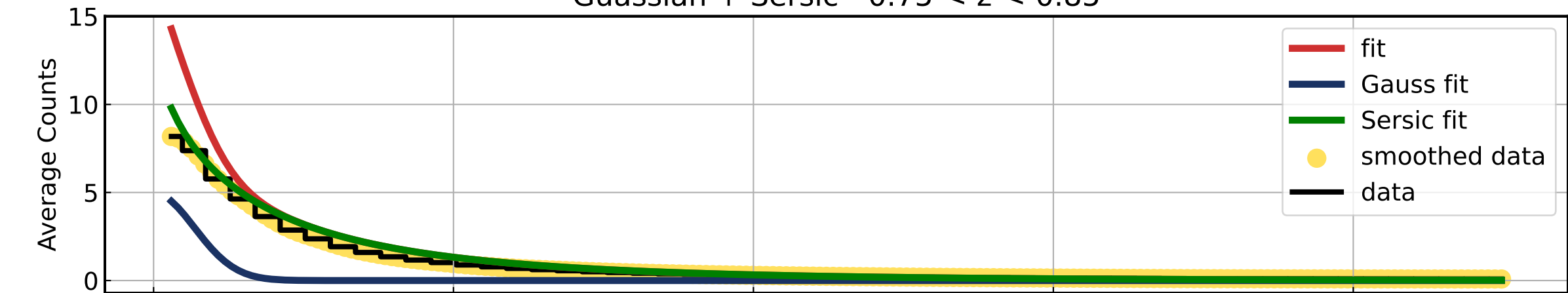
Guassian + Sersic - 0.75 < z < 0.85
