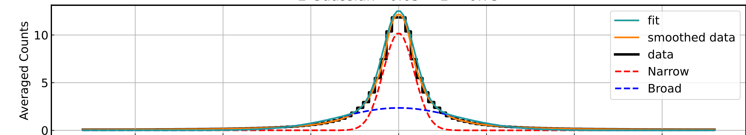
2 Guassian - 0.65 < z < 0.75
