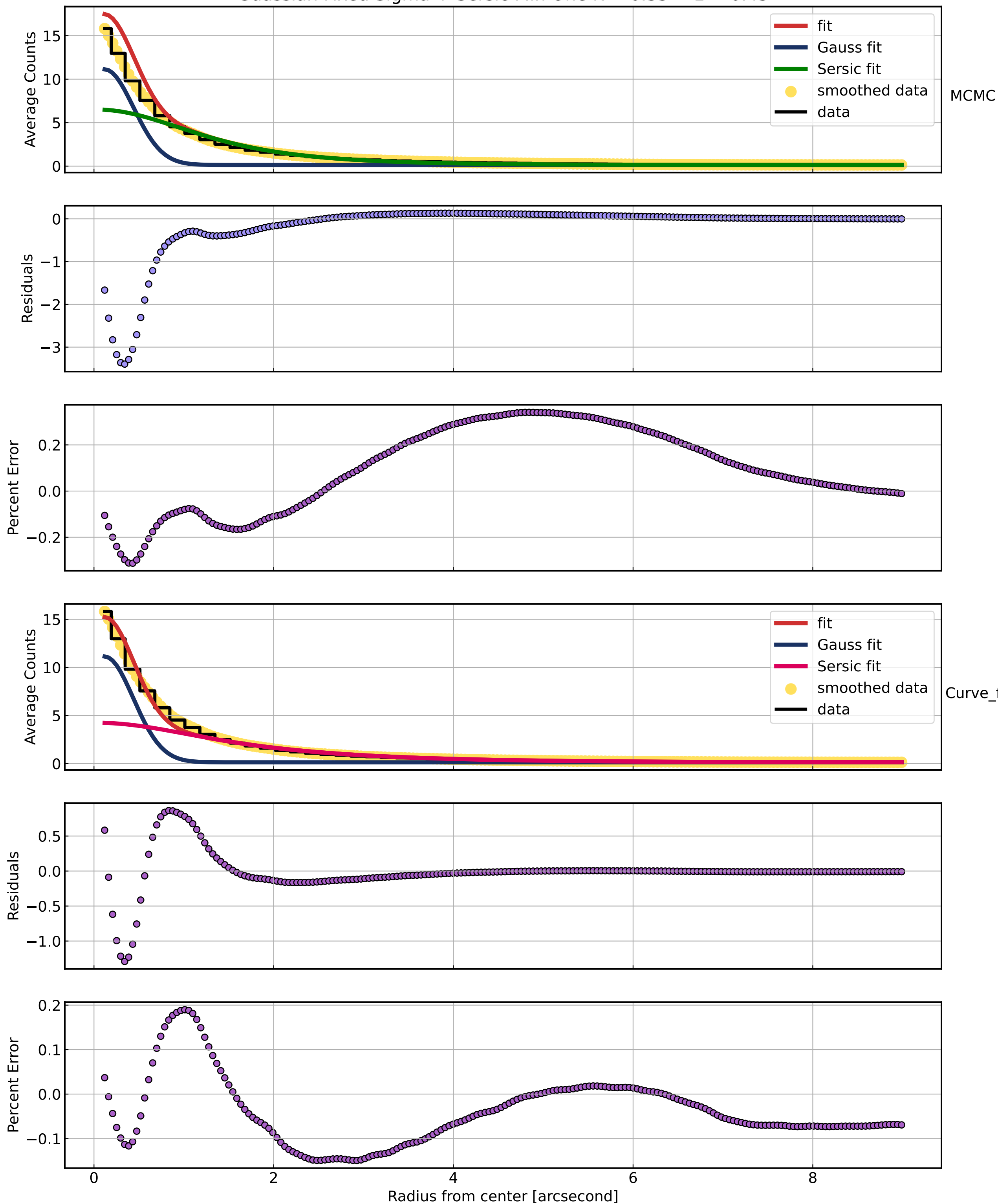
Guassian Fixed Sigma + Sersic Min One N -- 0.35 < z < 0.45
