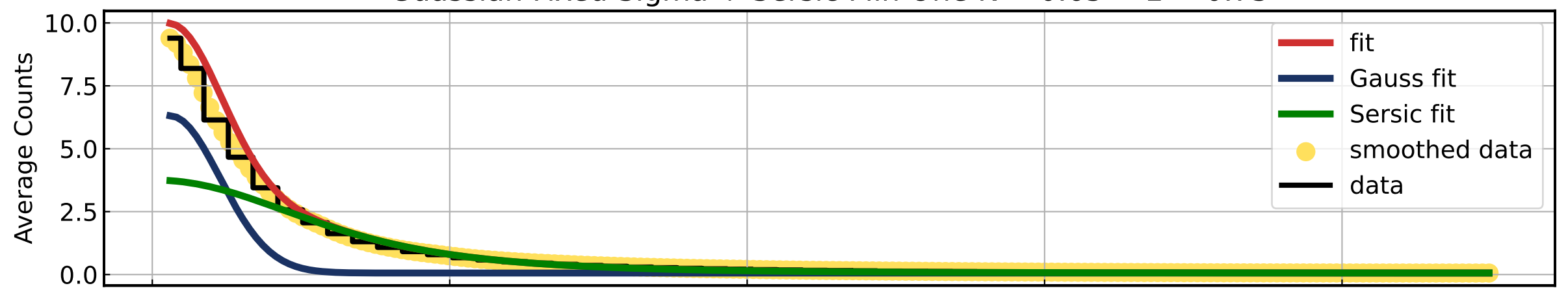
Guassian Fixed Sigma + Sersic Min One N -- 0.65 < z < 0.75
