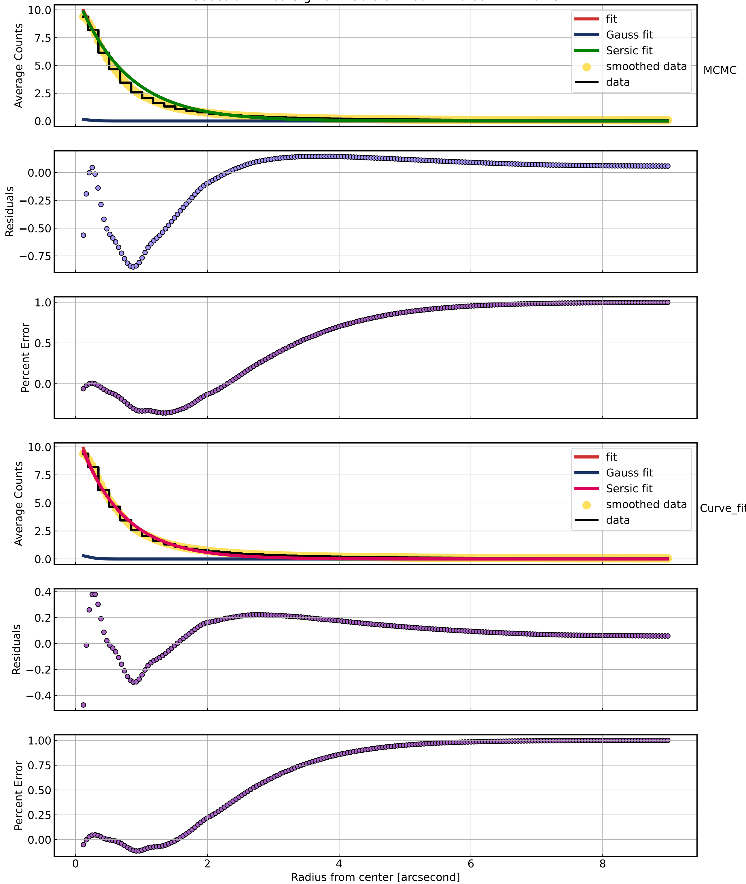
Guassian Fixed Sigma + Sersic Fixed N -- 0.65 < z < 0.75
