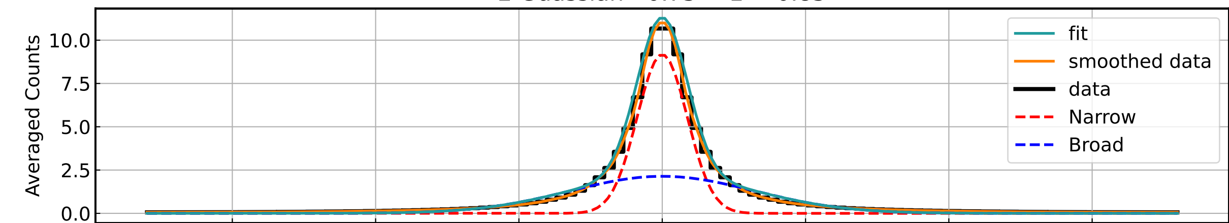
2 Guassian - 0.75 < z < 0.85
