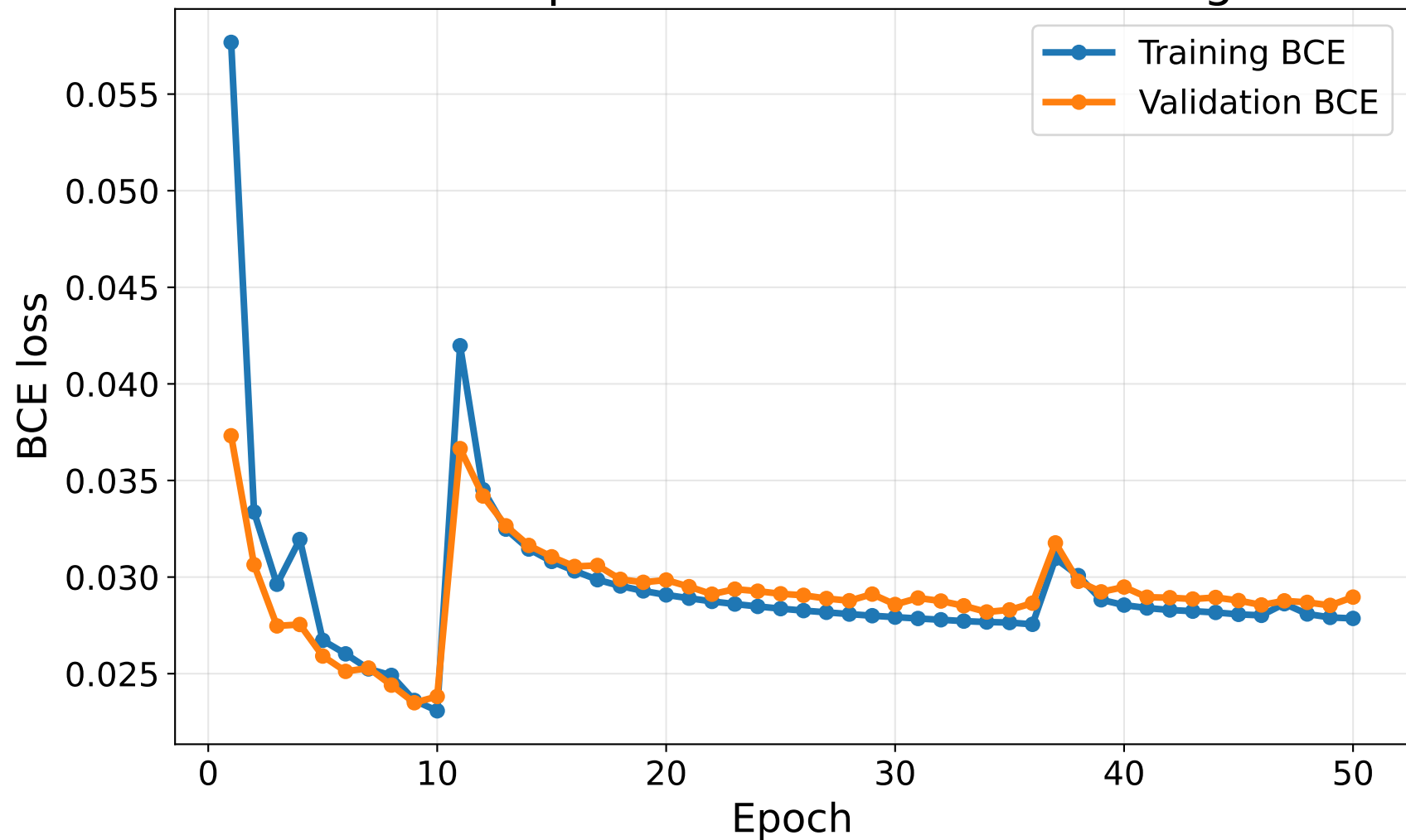
Full 128D Compound Autoencoder Training Curve
