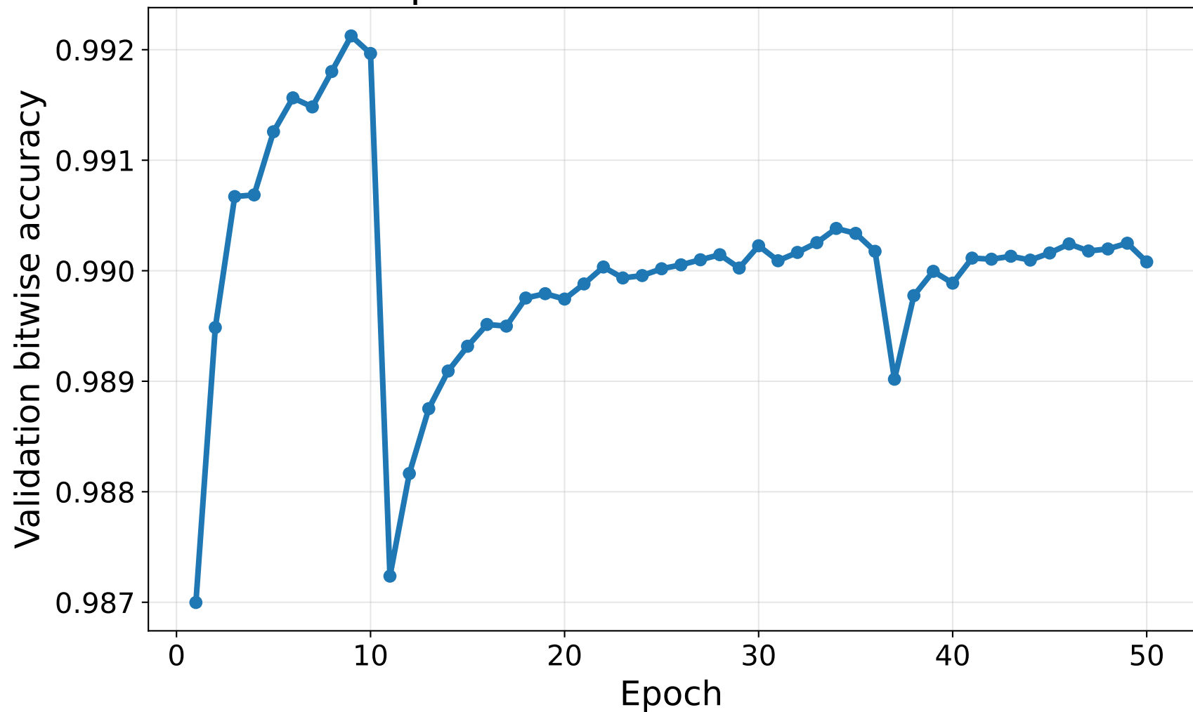
Full 128D Compound Autoencoder Validation Accuracy
