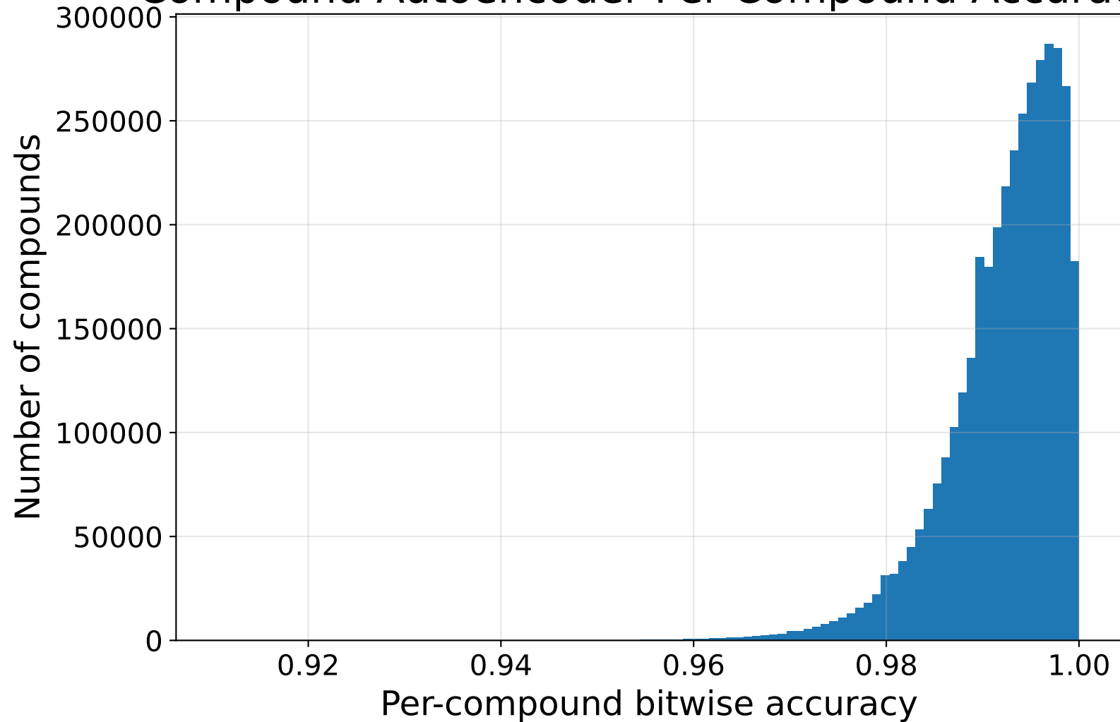
Compound Autoencoder Per-Compound Accuracy
