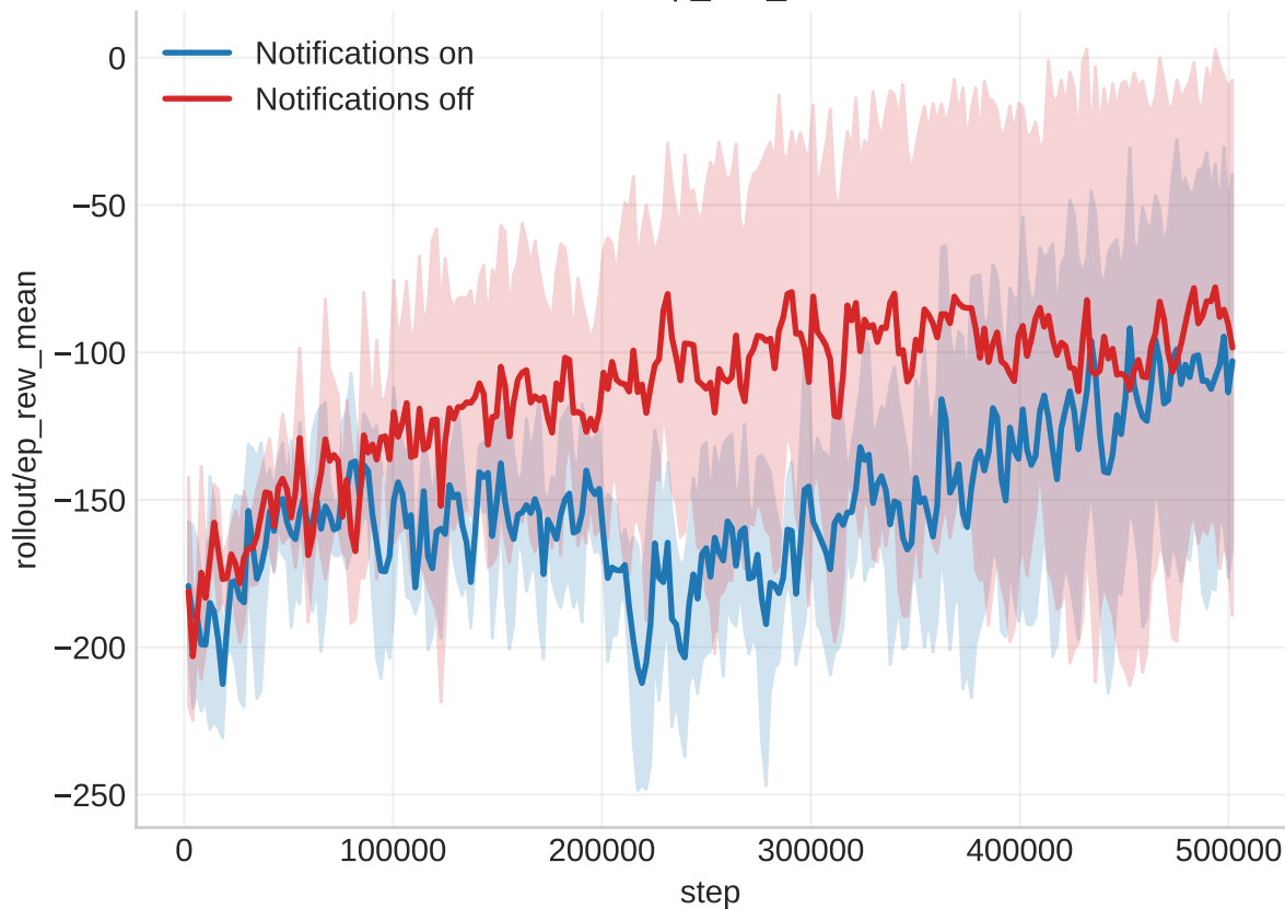
rollout/ep_rew_mean
