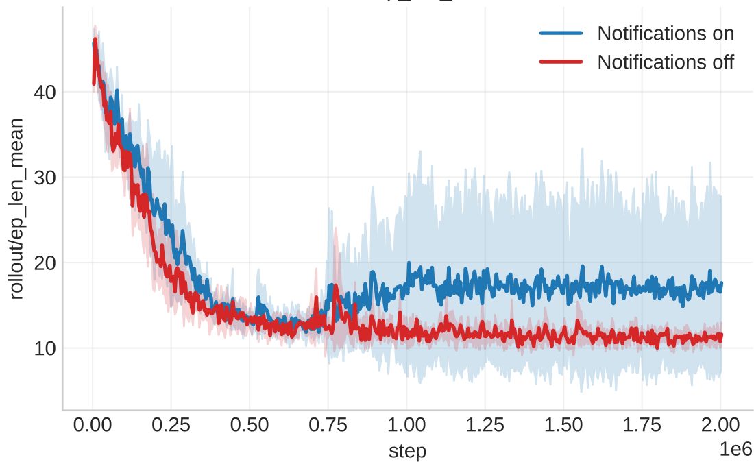
rollout/ep_len_mean
