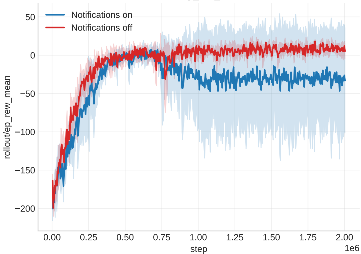
rollout/ep_rew_mean
