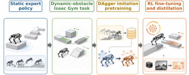
Fig. 1. Current training pipeline. A static-terrain expert initializes dynamic-obstacle learning through DAgger imitation pretraining, after which the policy is fine-tuned by the original base RL stage and later prepared for camera distillation.
