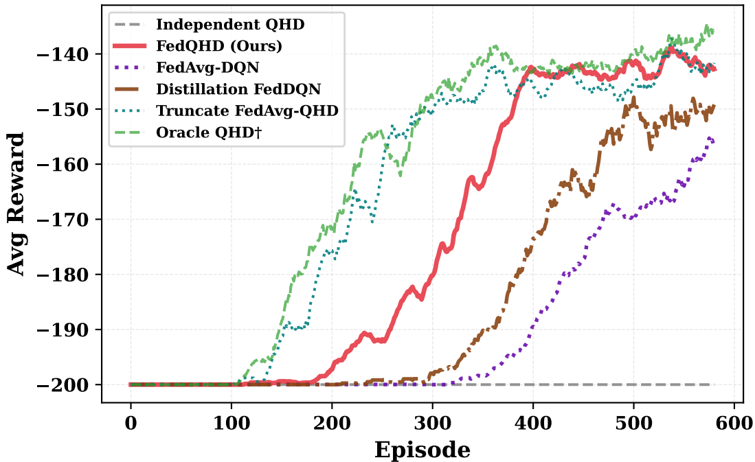
MountainCar-v0 — Q1: Homogeneous Encoders
