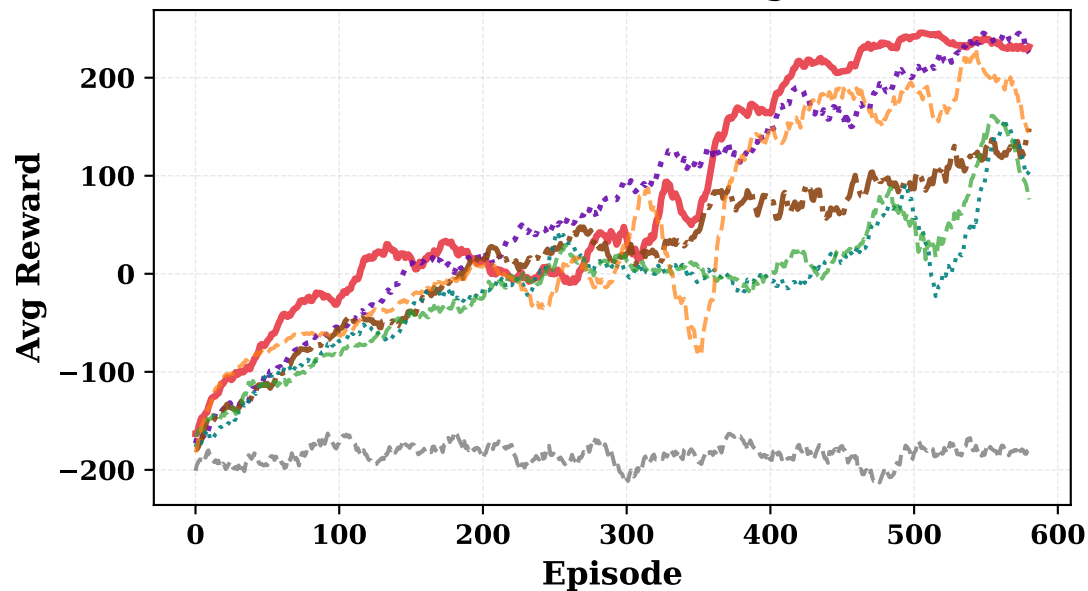
(c) LunarLander — Homogeneous
