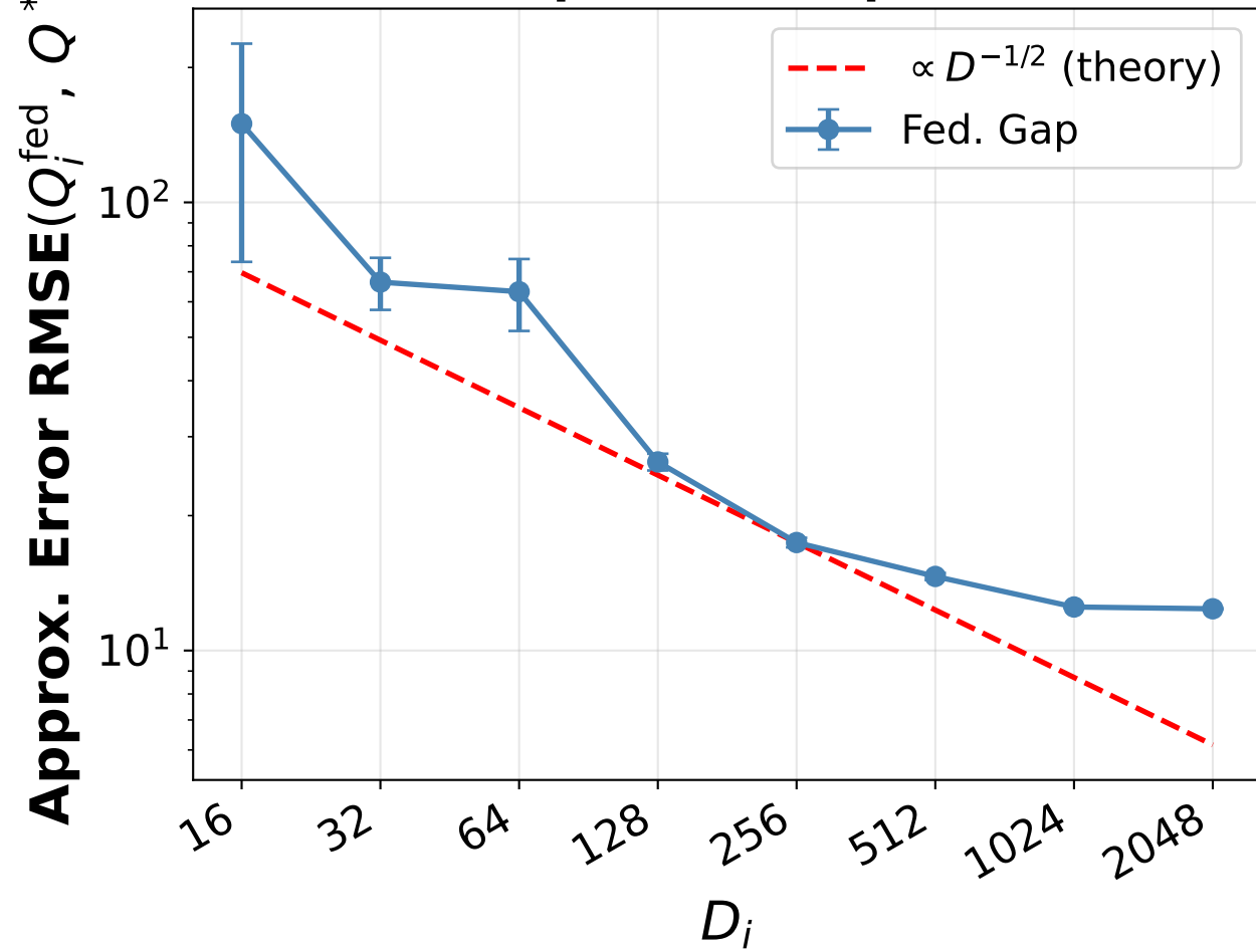
Fed. Gap vs D_i (slope -0.53)
