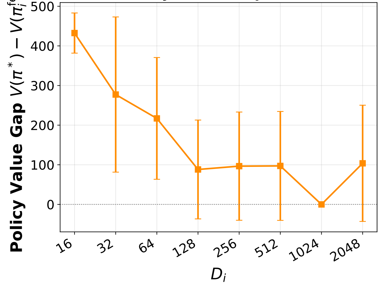
Policy Value (Gap) vs D_i
