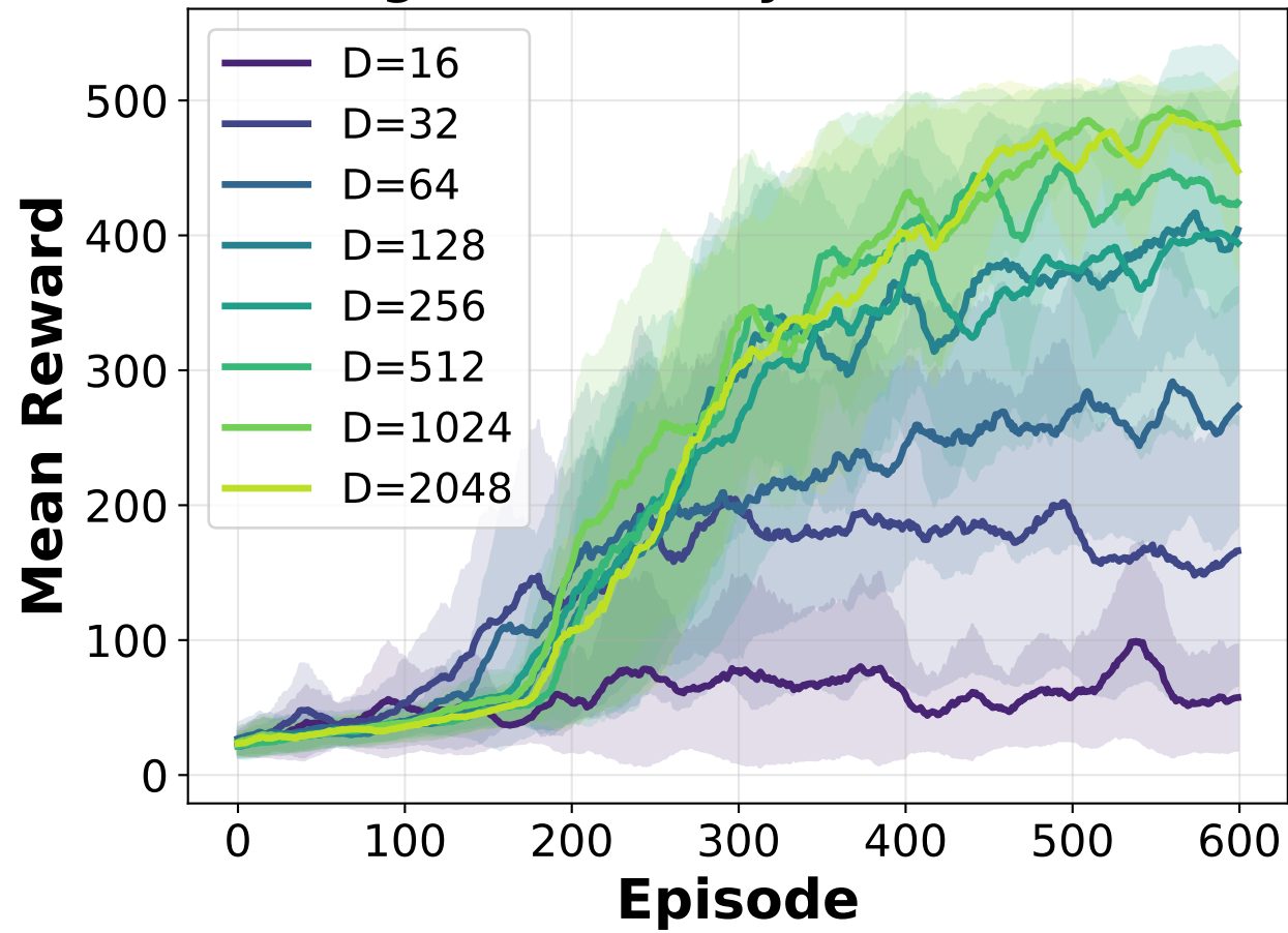
Learning Curves (vary D , m=64 ) ( w=20 )
