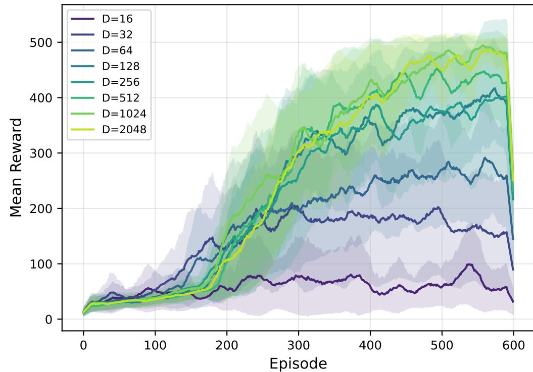
Learning Curves (vary D, m=64) (w=20)
