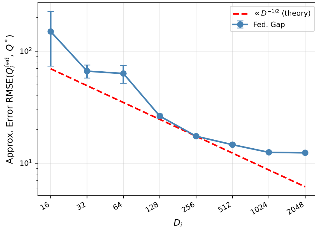
Fed. Gap vs D_i (slope -0.53)
