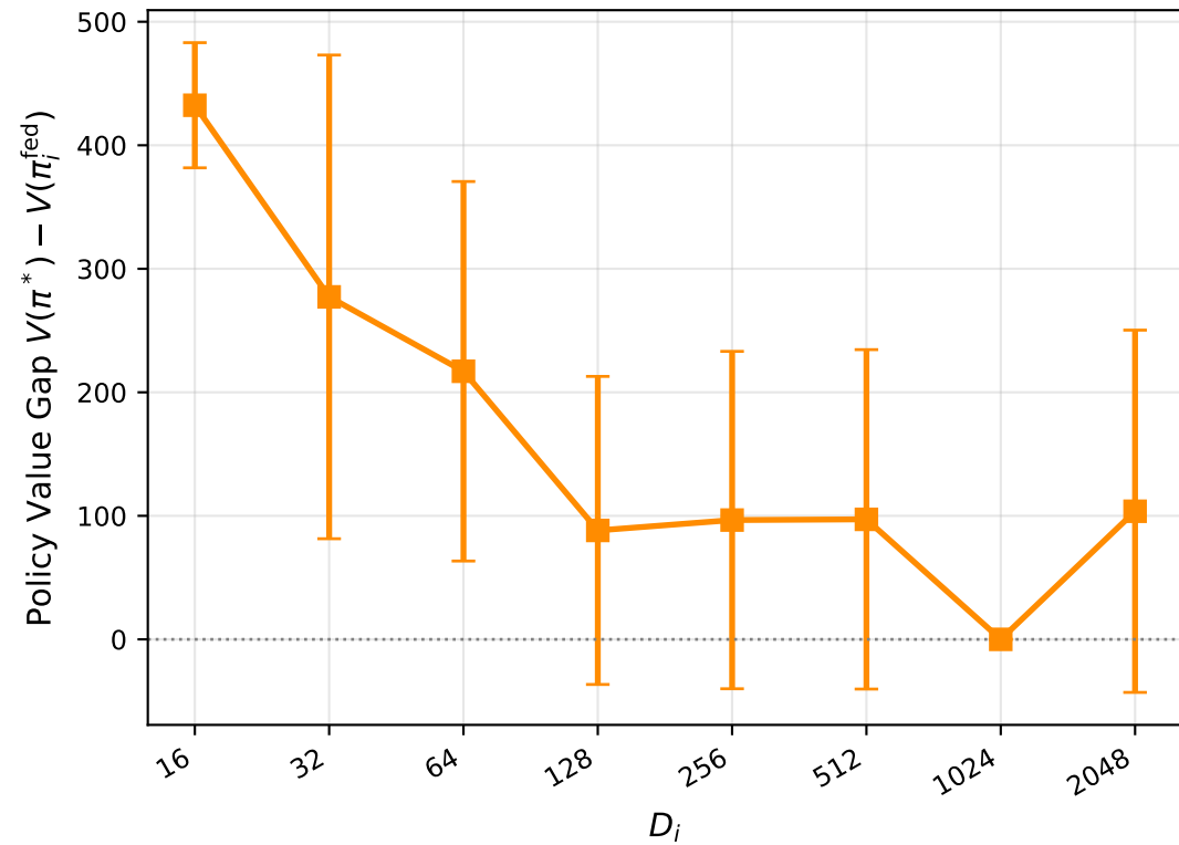
Policy Value (Gap) vs D_i
