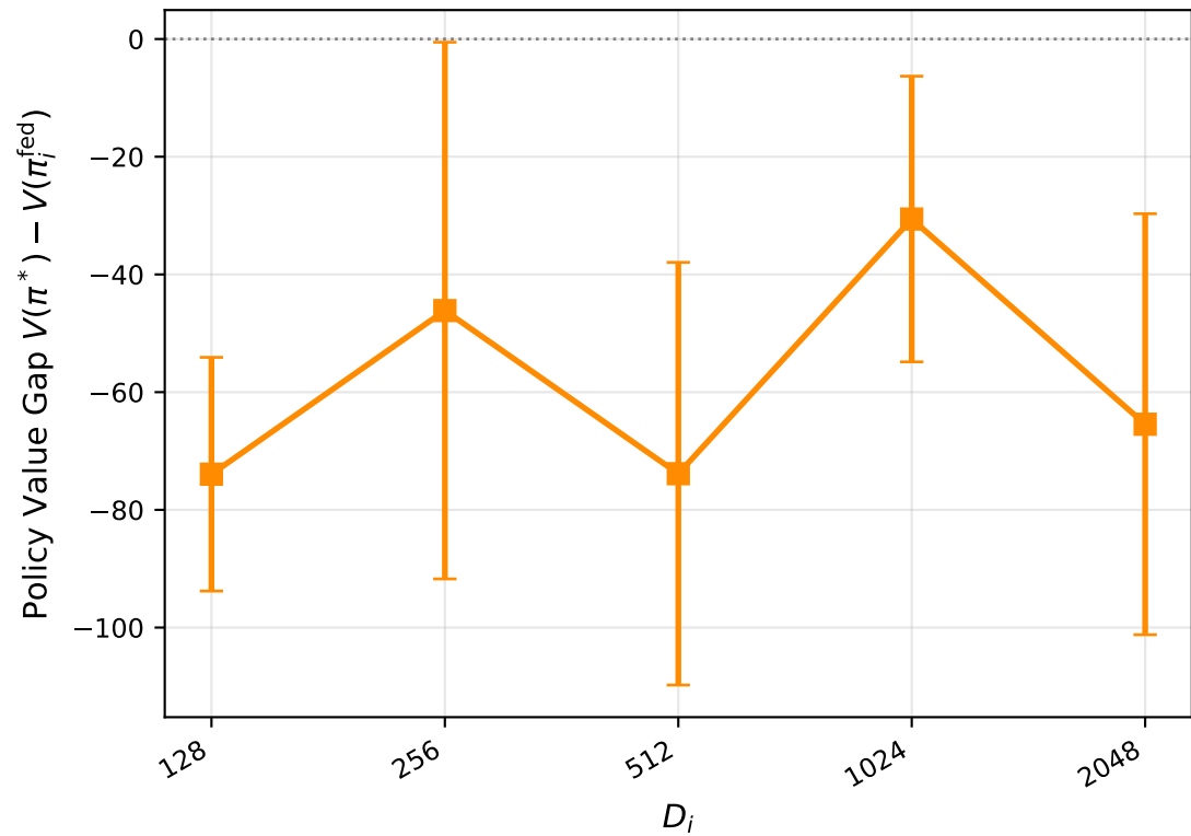
Policy Value (Gap) vs D_i
