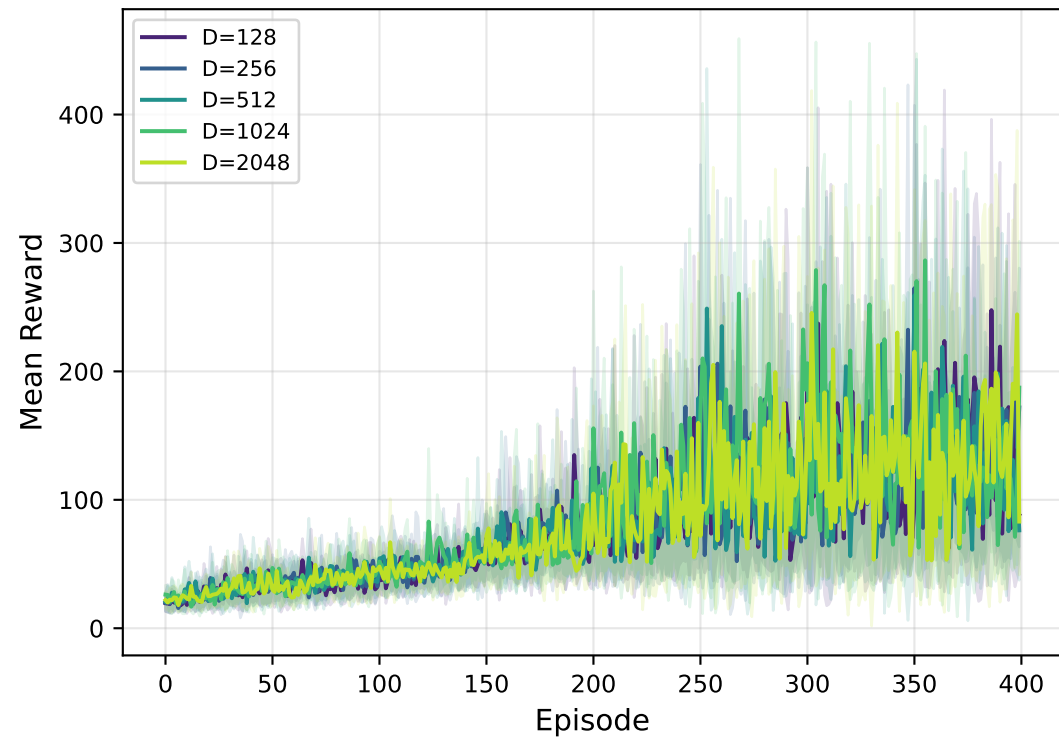
Learning Curves (vary D, m=8192)
