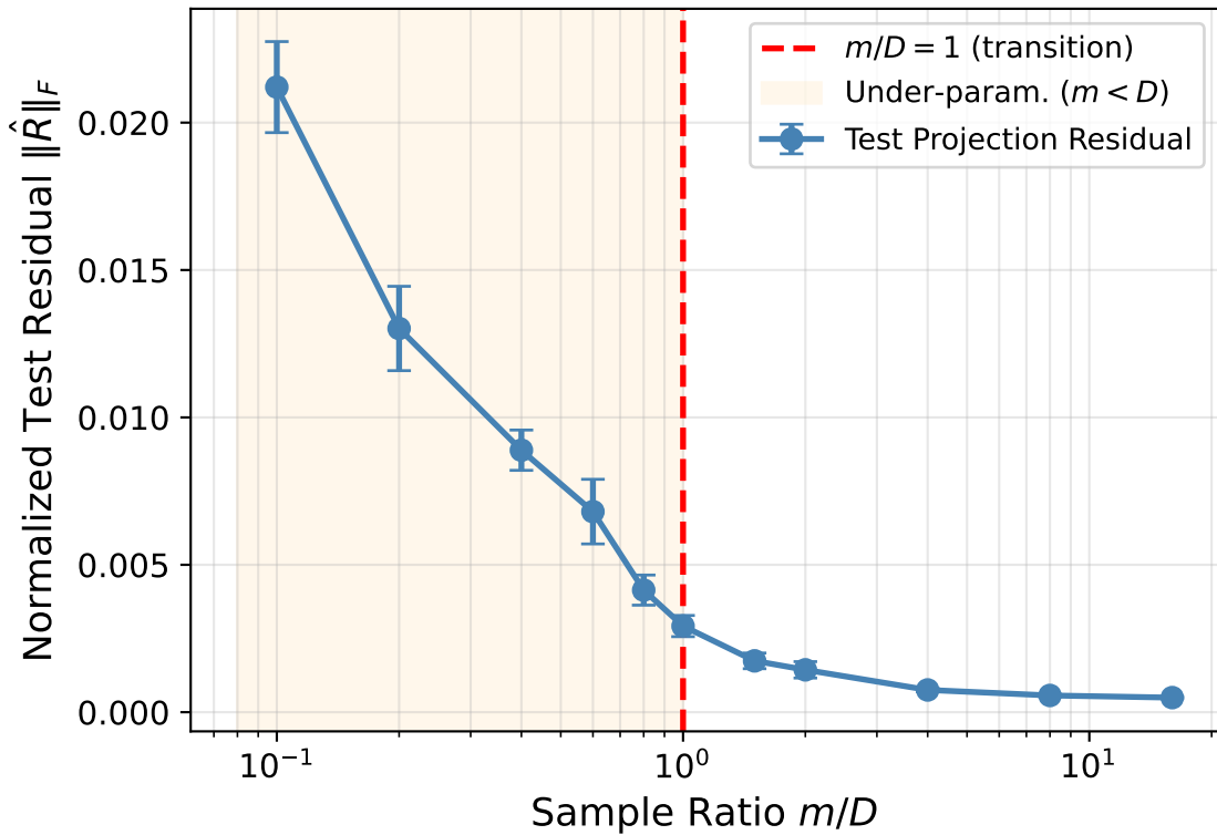
Ablation 2: Sample Regime Transition ( D = 512 )
