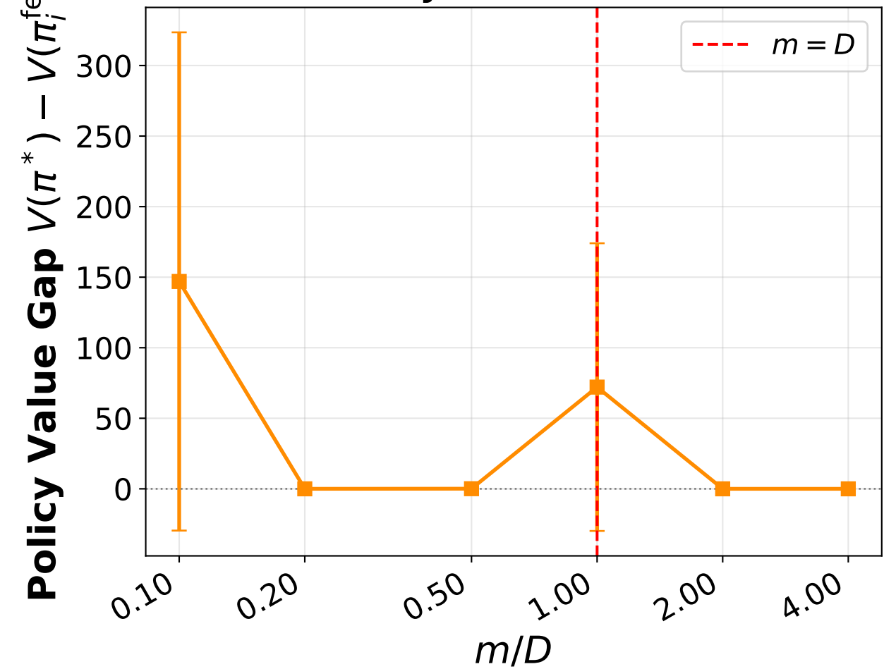
Policy Value vs m/D
