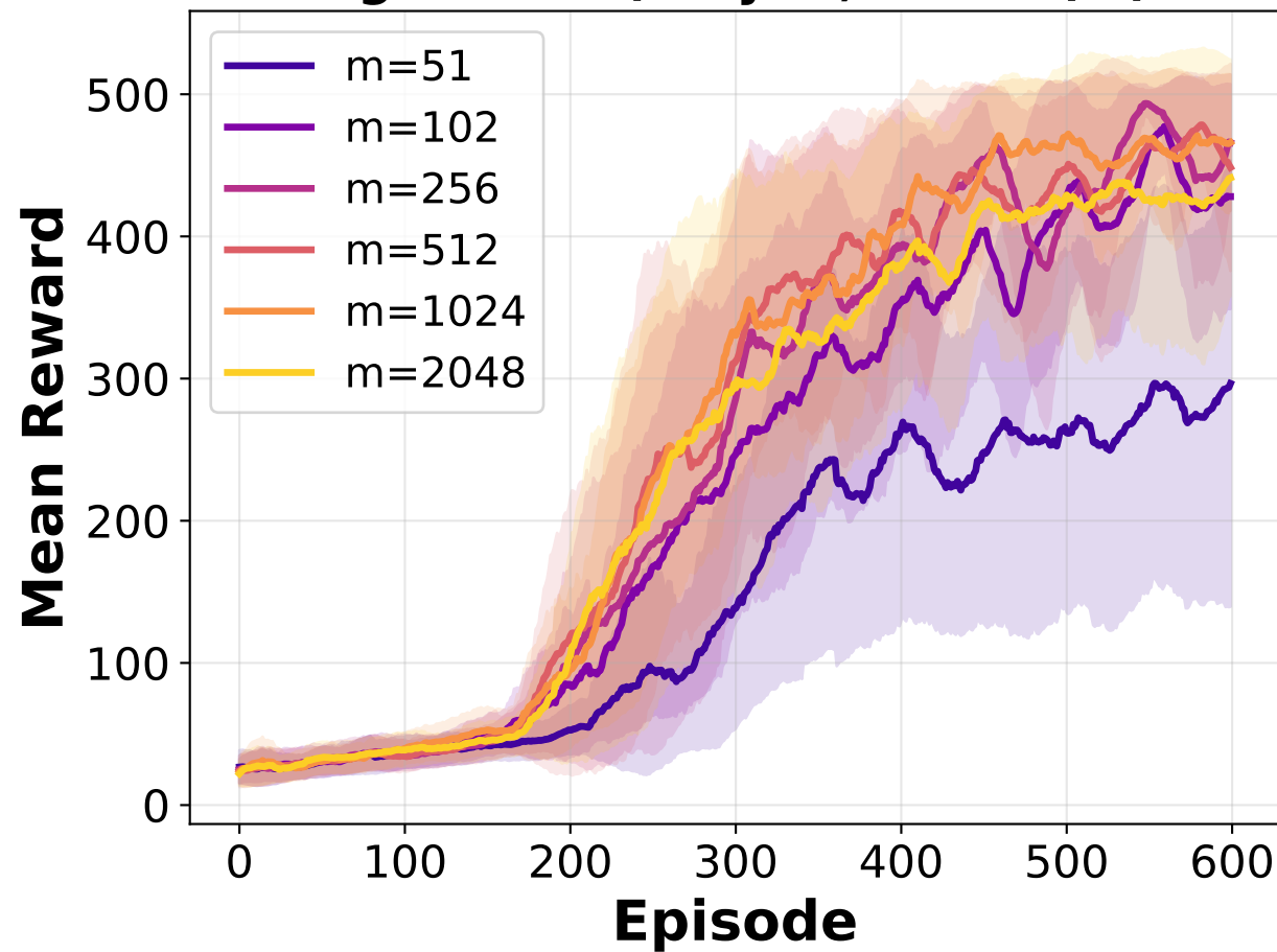
Learning Curves (vary m , D=512 ) ( w=20 )
