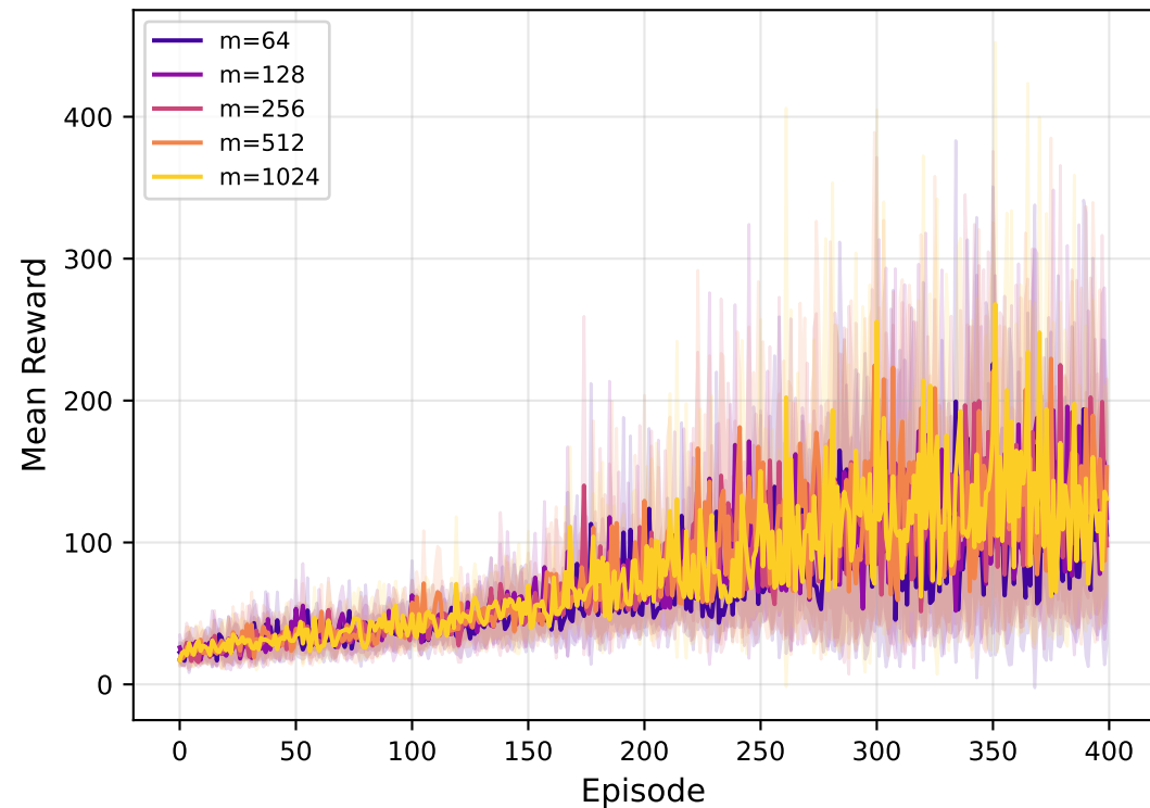
Learning Curves (vary m , D=512 )
