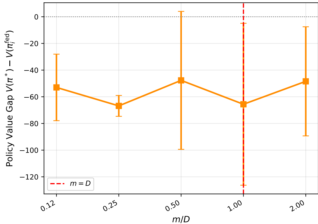
Policy Value vs m/D
