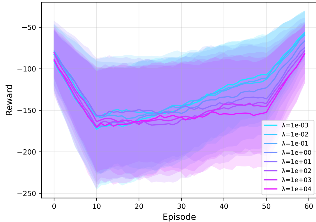
Learning Curves (vary \lambda , D=1024 , m=256 ) ( w=20 )
