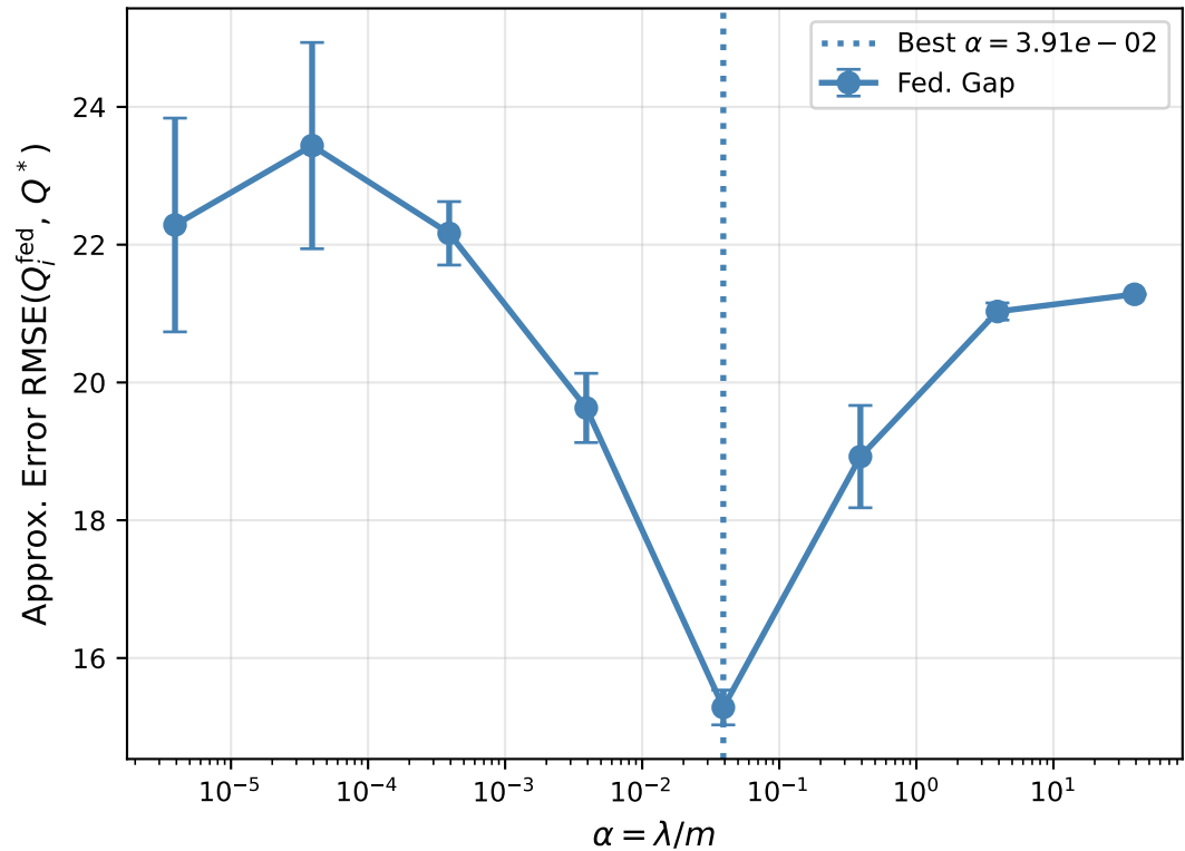
Fed. Gap vs \alpha ( D=1024 , m=256 )
