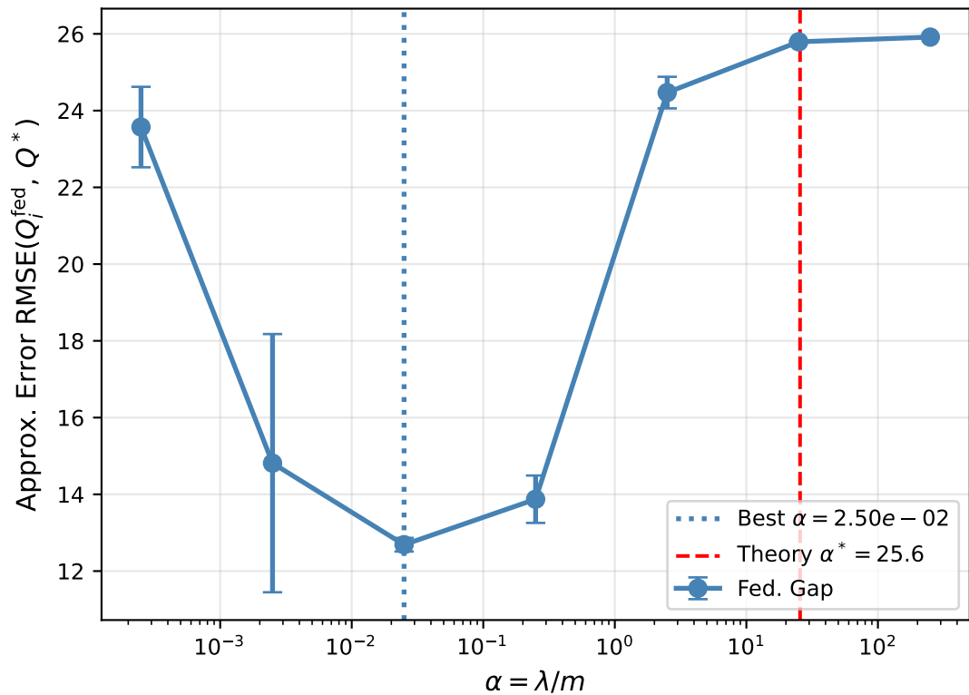
Fed. Gap vs \alpha ( D=512 , m=400 )
