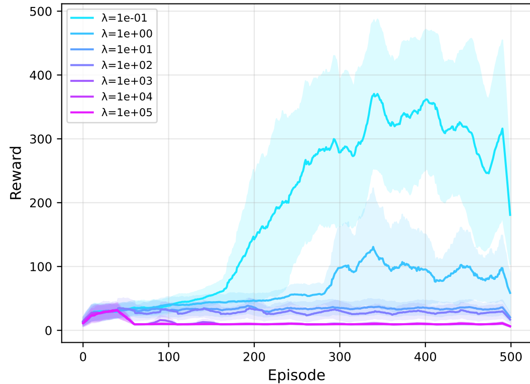
Learning Curves (vary \lambda , D=1024 , m=512 ) ( w=20 )
