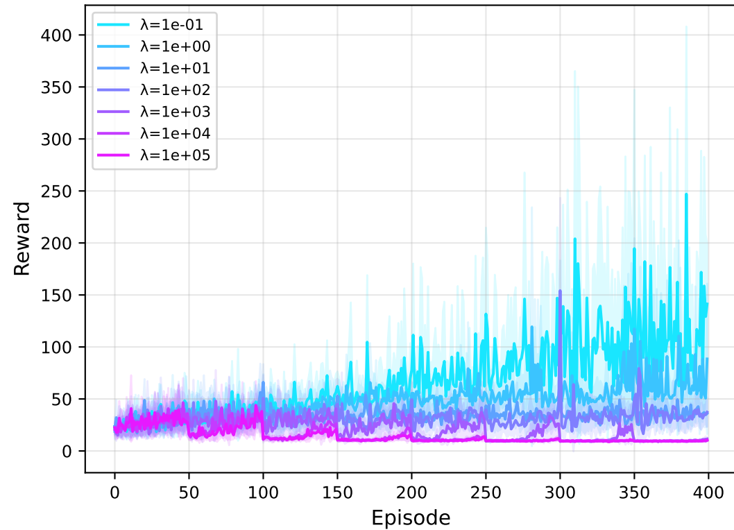
Learning Curves (vary \lambda , D=512 , m=400 )
