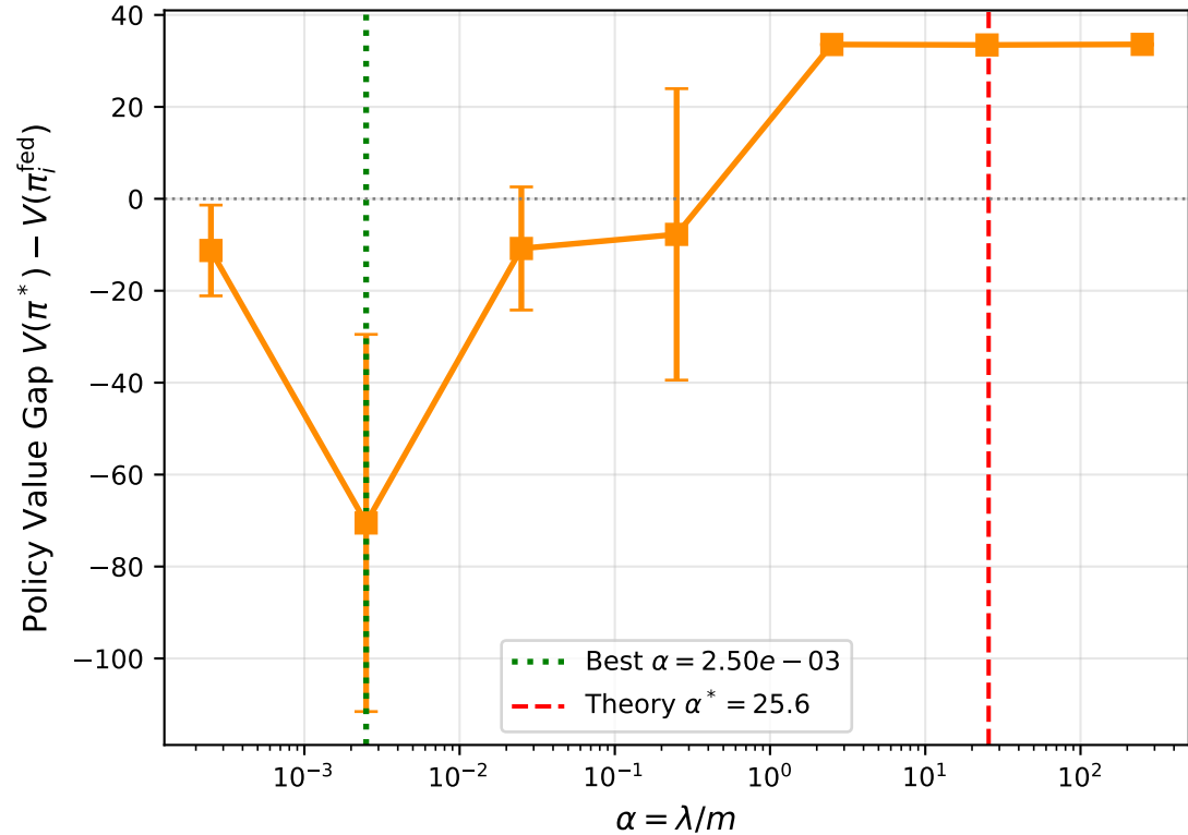
PV vs \alpha ( D=512 , m=400 )
