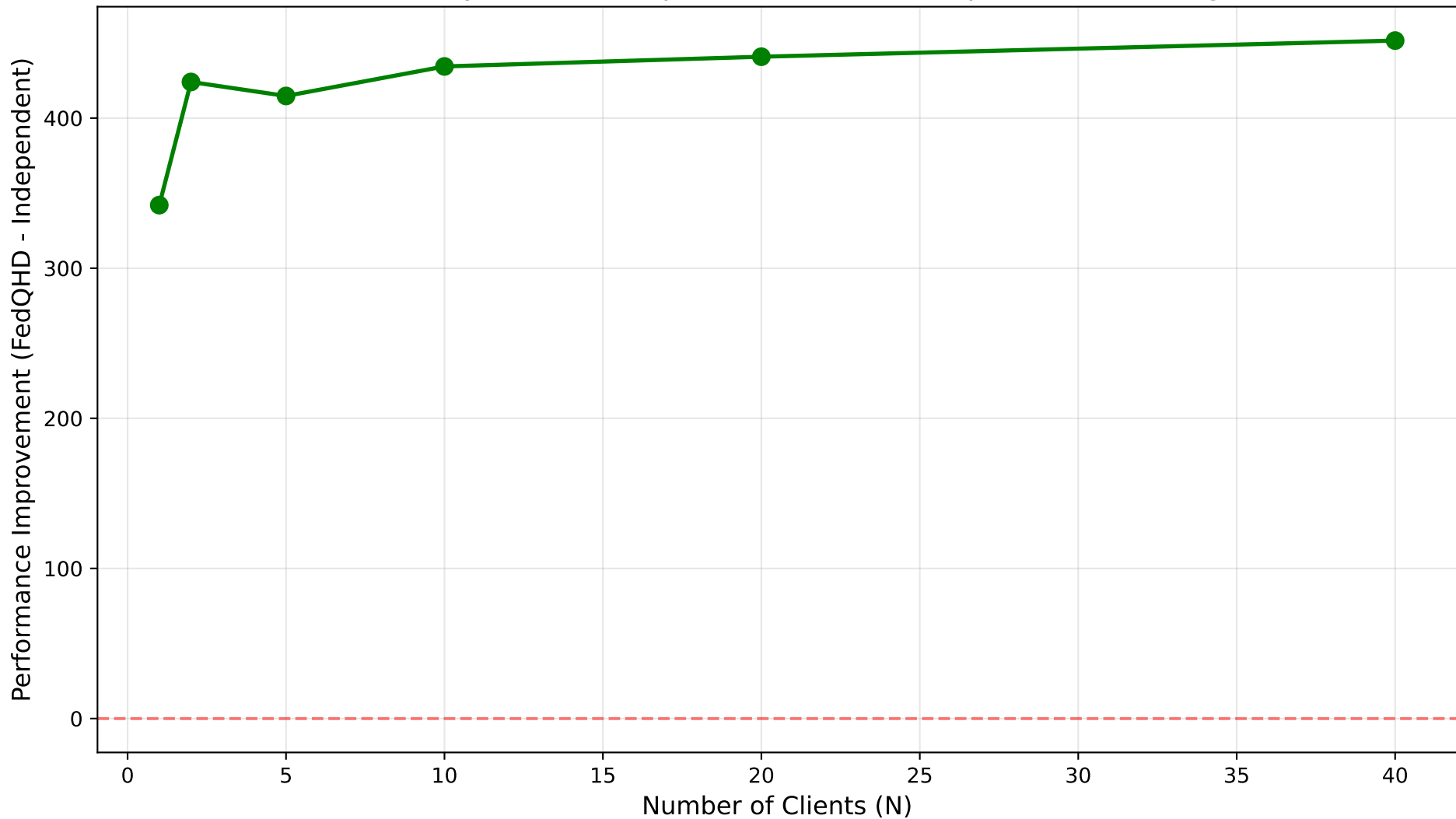
Scalability: FedQHD Improvement over Independent Learning
