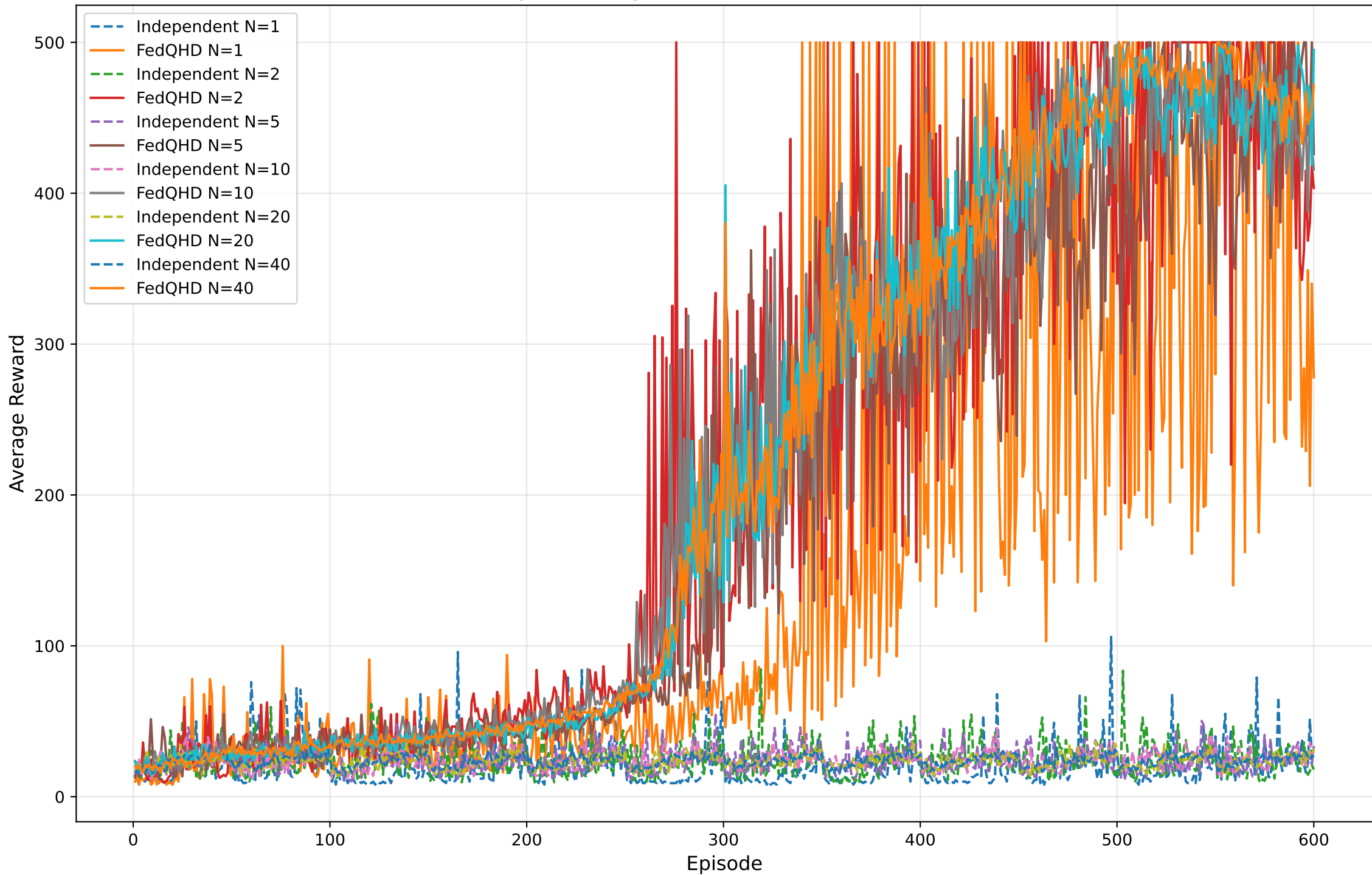
Scalability: Learning Curves for Different Client Counts
