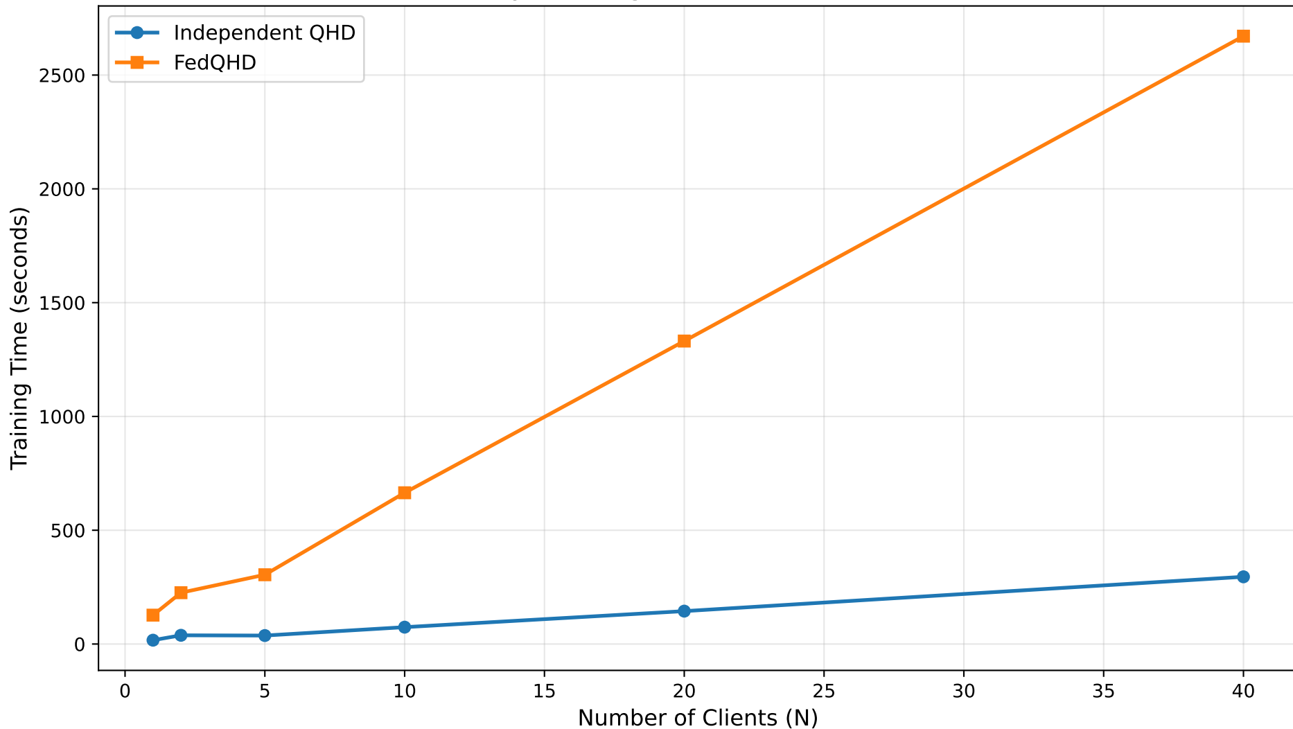
Scalability: Training Time vs. Number of Clients
