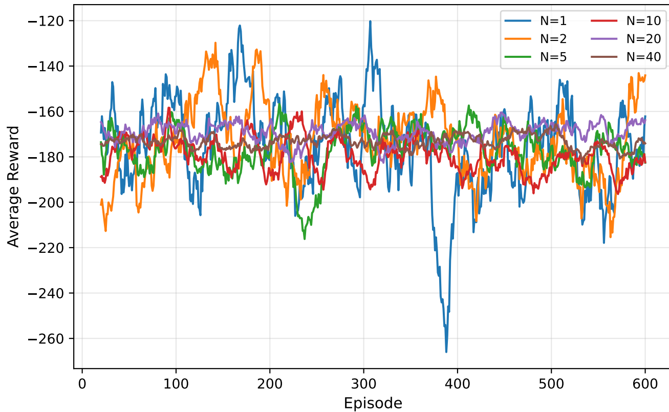
Independent QHD
