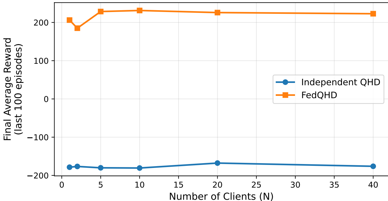
Scalability: Performance vs. Number of Clients
