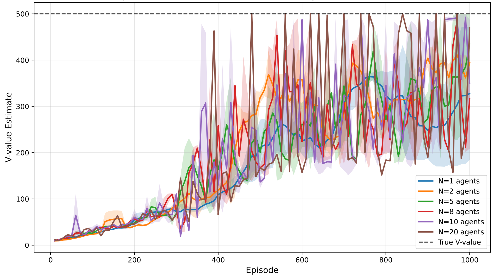
Agent Number Ablation: V-value Learning Curves (D=10000)
