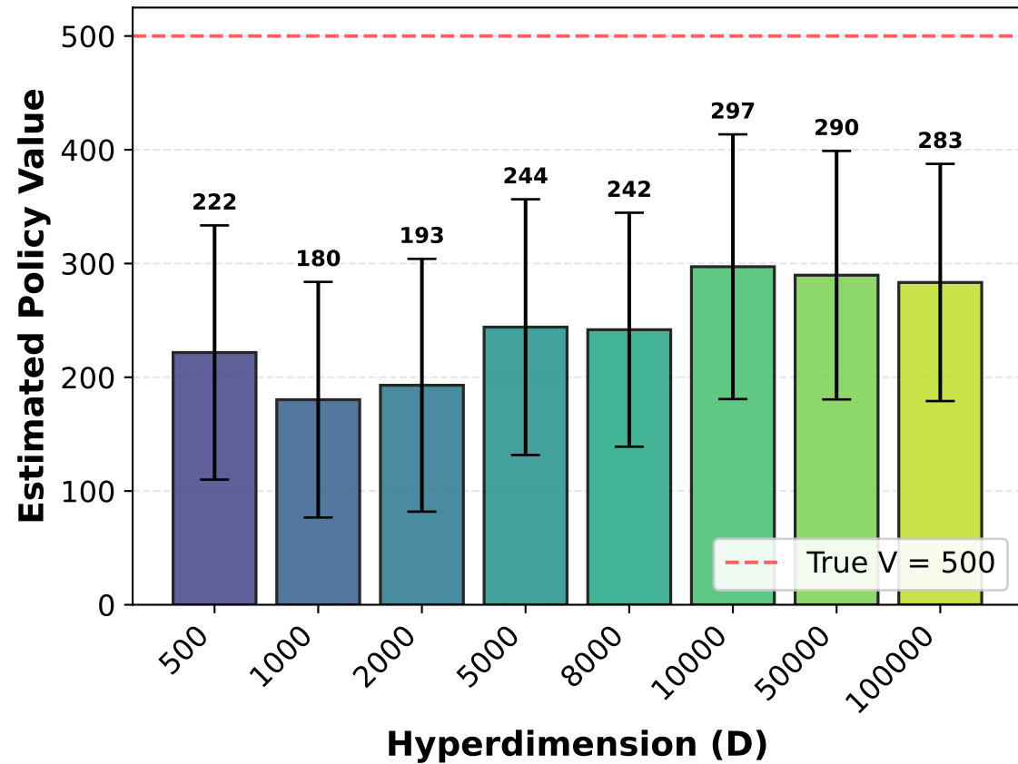
Episodes 800-1200
