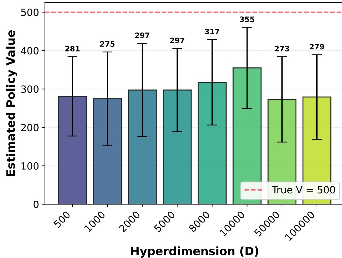
Episodes 1000-1500
