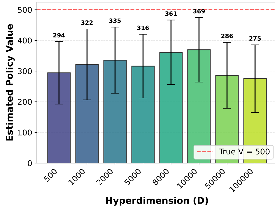
Episodes 1200-1600
