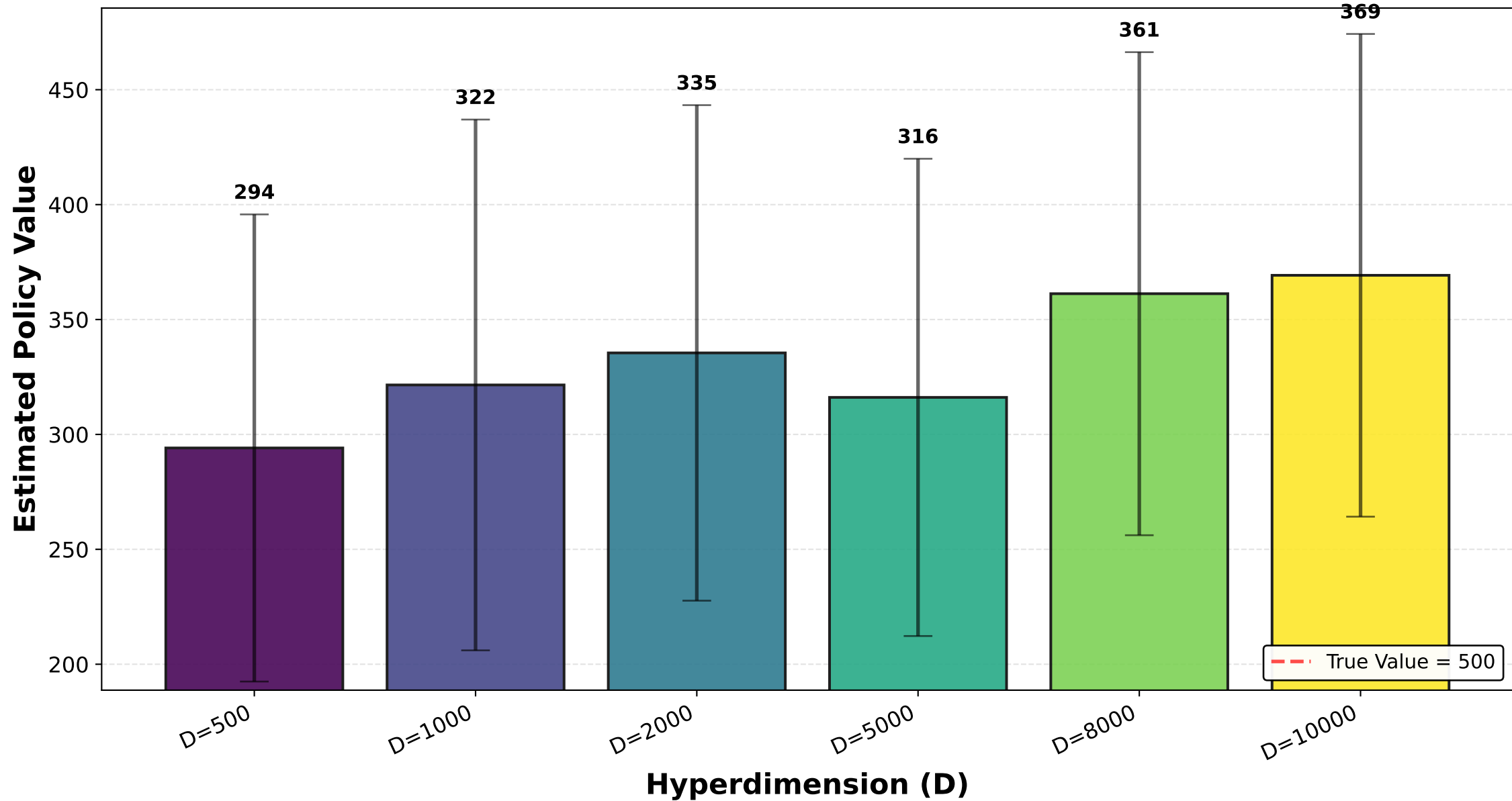
Policy Value vs Hyperdimension (Episodes 1200-1600)
