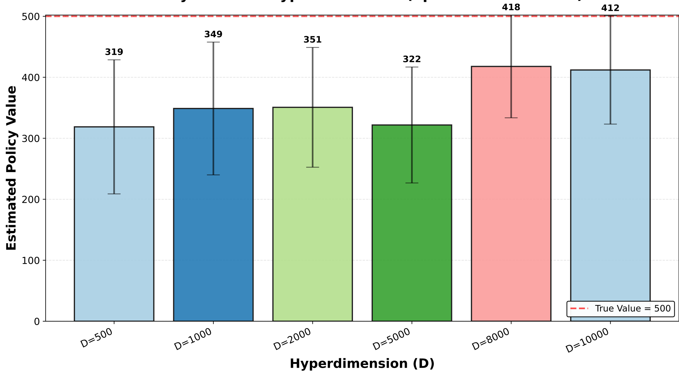
Policy Value vs Hyperdimension (Episodes 1450-1550)
