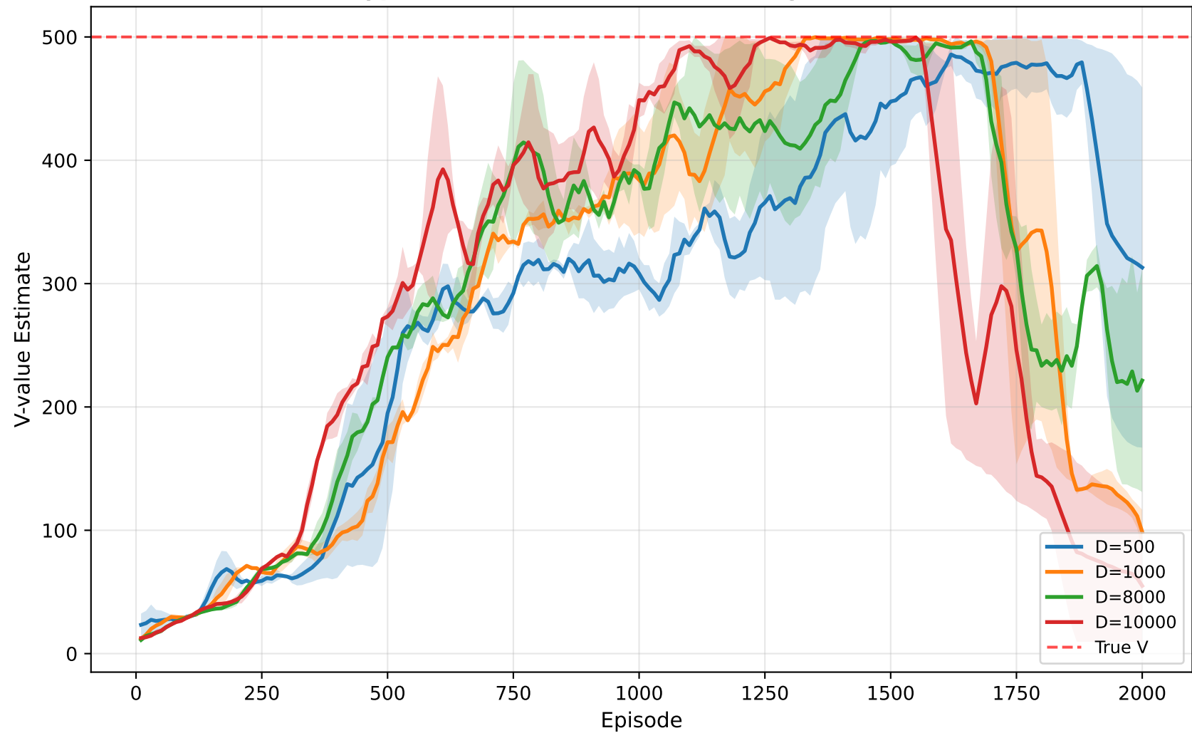
(c) Hyperdimension Ablation: Learning Curves (N=2)
