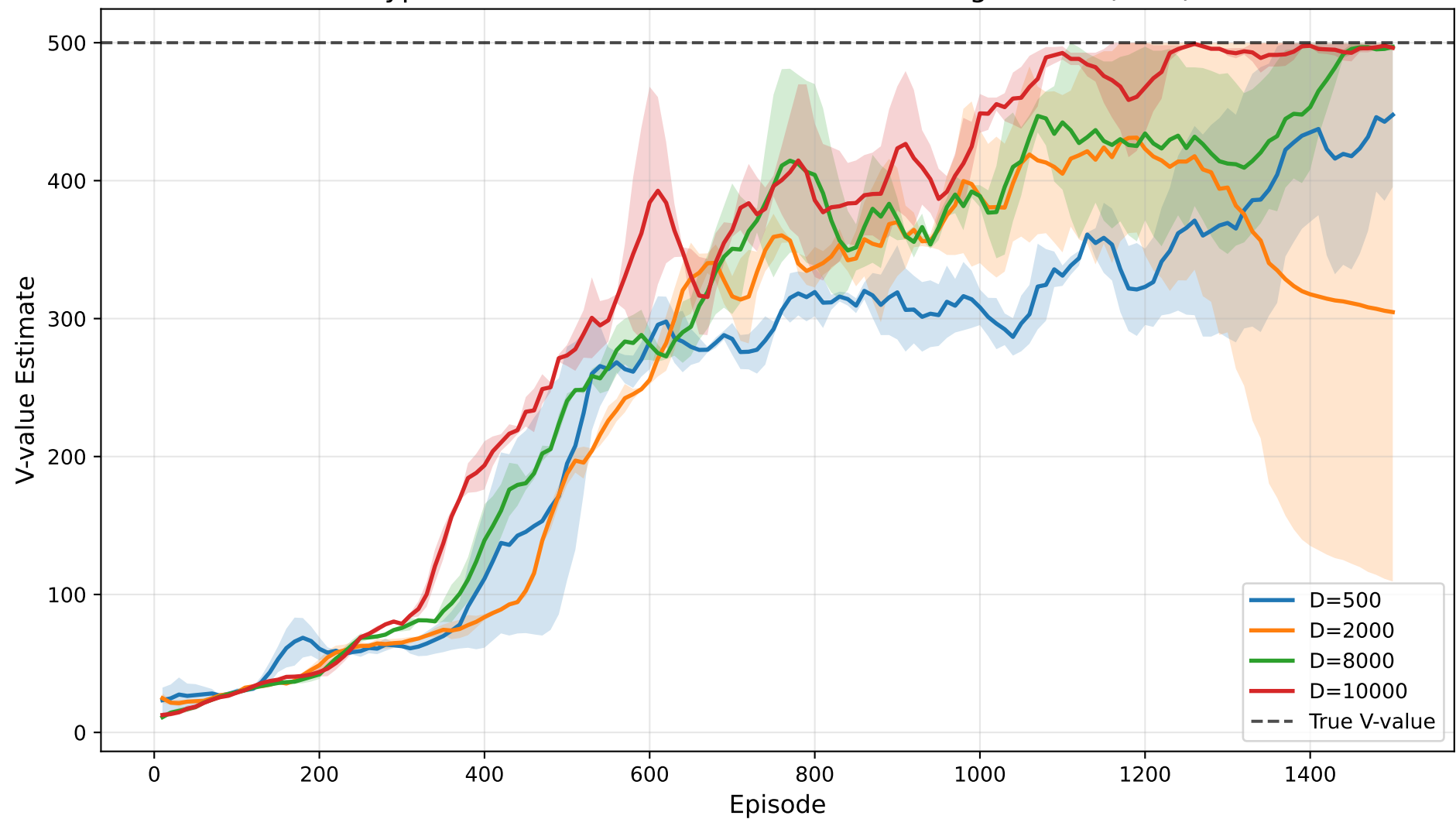
Hyperdimension Ablation: V-value Learning Curves (N=2)
