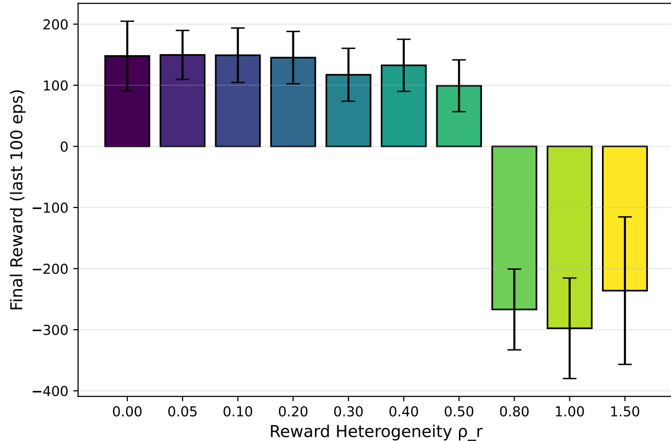
Final Performance by Heterogeneity Level
