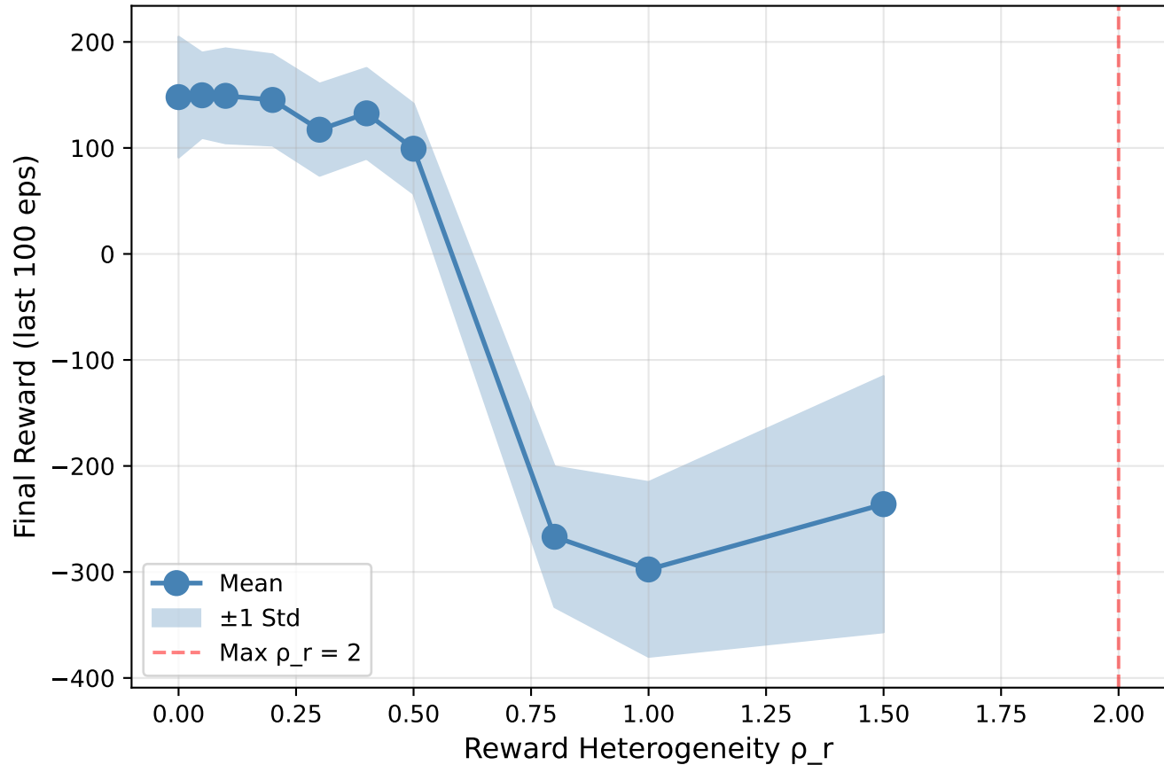
Performance Degradation vs Heterogeneity
