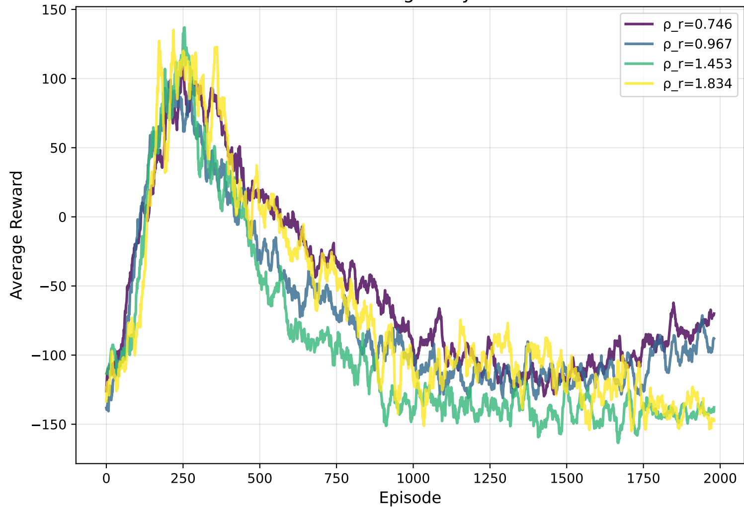
FedAvg HD-SARSA on LunarLander Reward Heterogeneity Ablation
