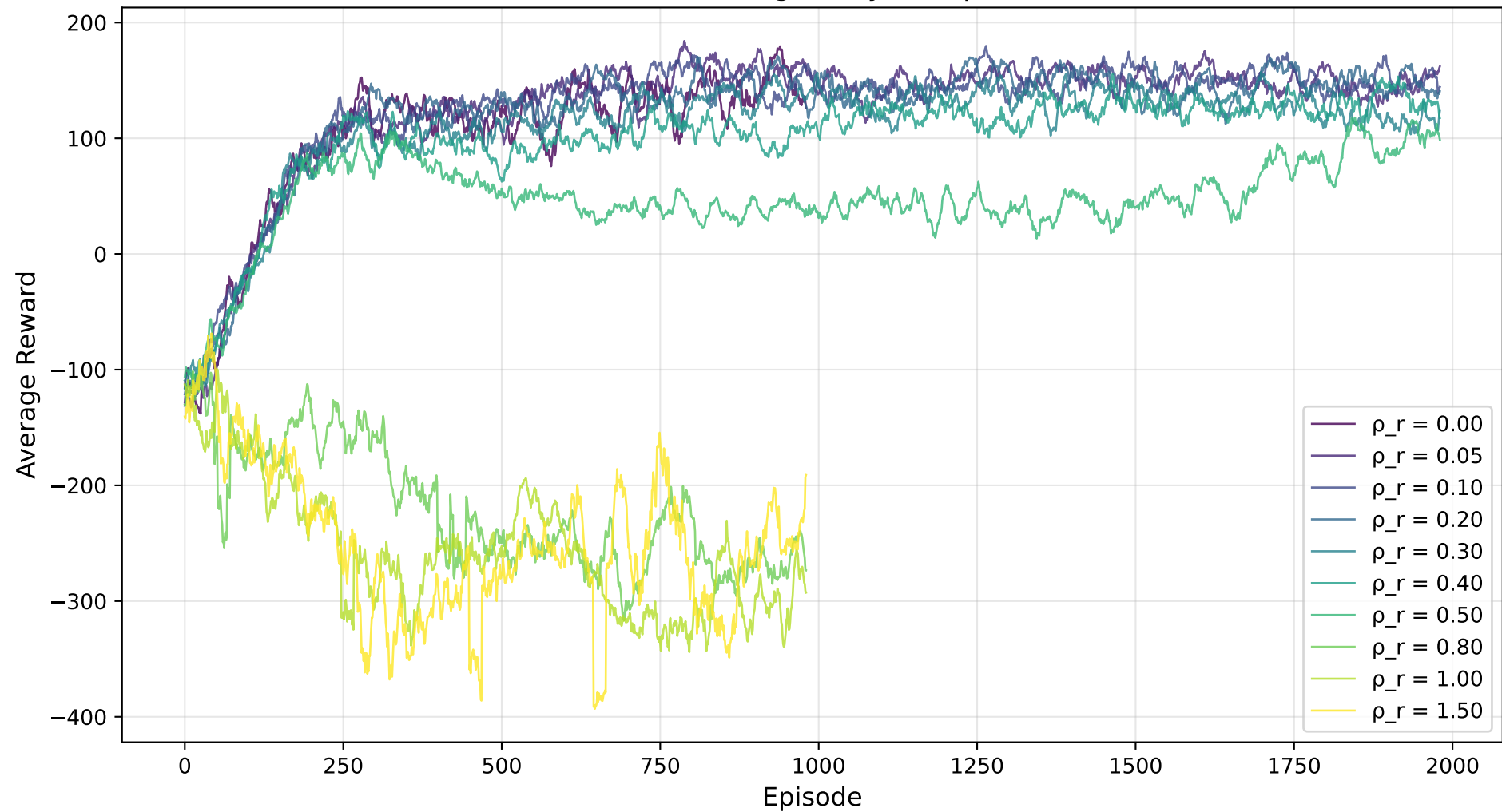
FedAvg HD-SARSA on LunarLander Reward Heterogeneity Comparison
